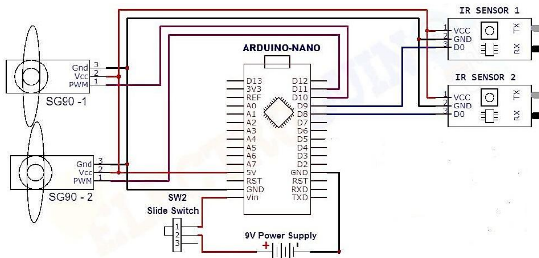
Figure 2. Circuit diagram.
