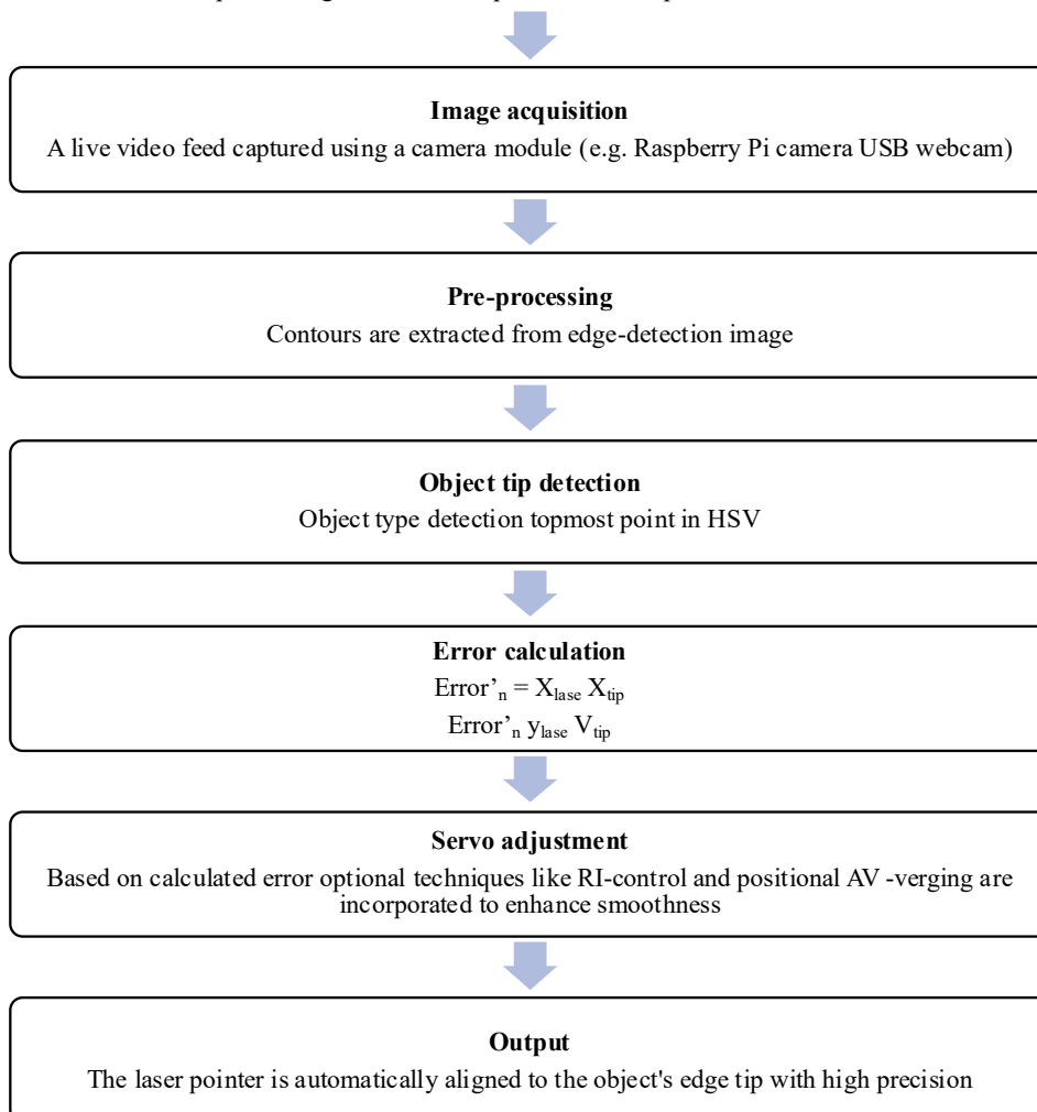
Figure 7. Flow of technology used for laser adjustment.
