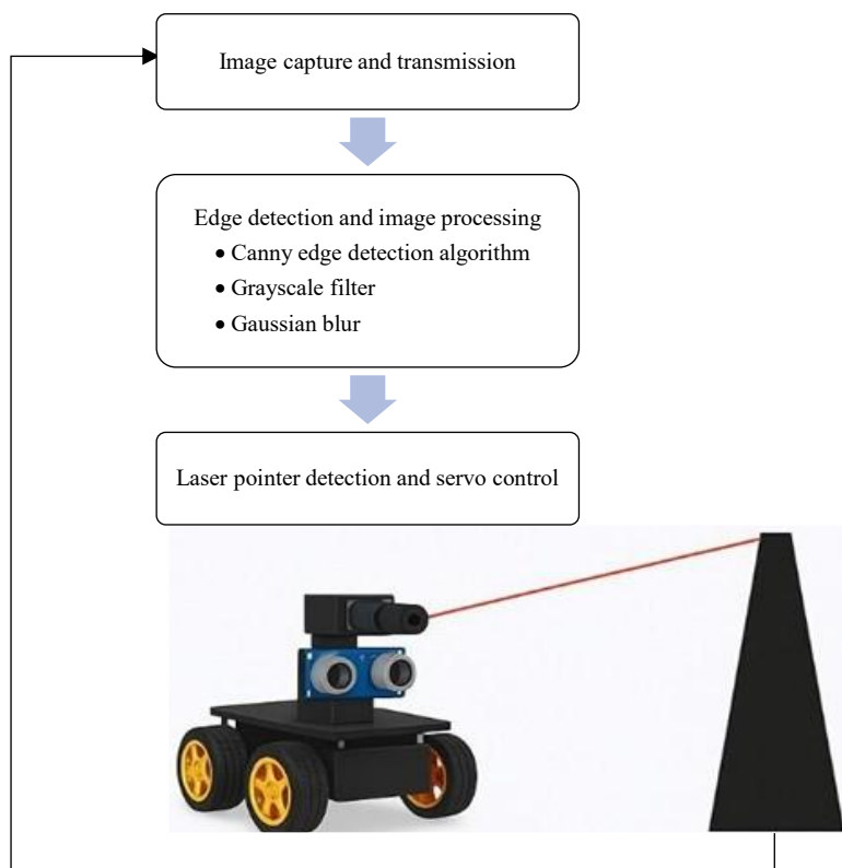
Figure 1. Short flow diagram of how Xypher Bot works.
