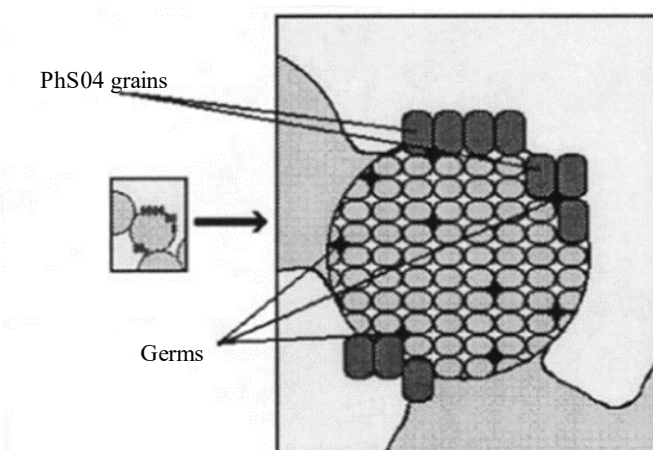
Figure 4. PbO 2 Transformation with a high current discharge [13].
