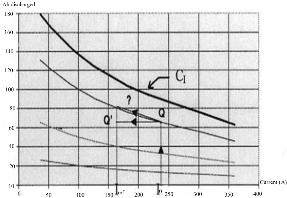
Figure 7. Capacity evolution for a 6RGT180 battery at 25 C [16].
