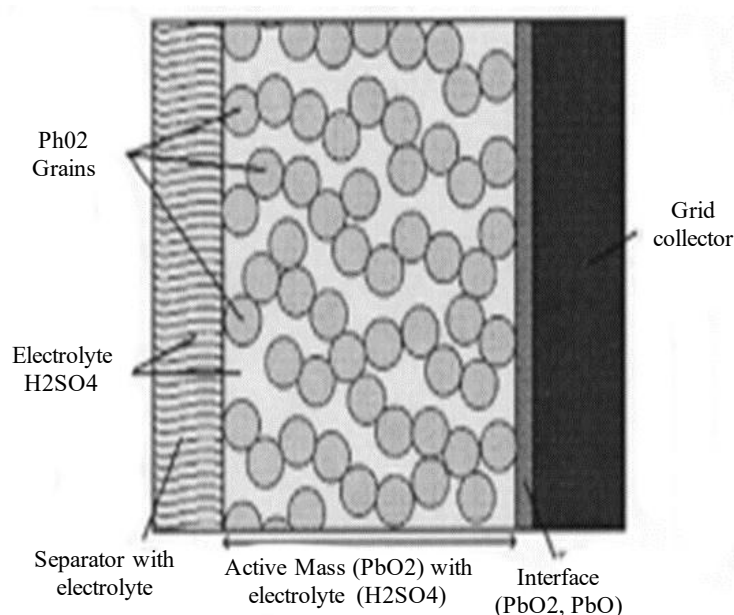
Figure 1. Section view of the positive plate.[10].
