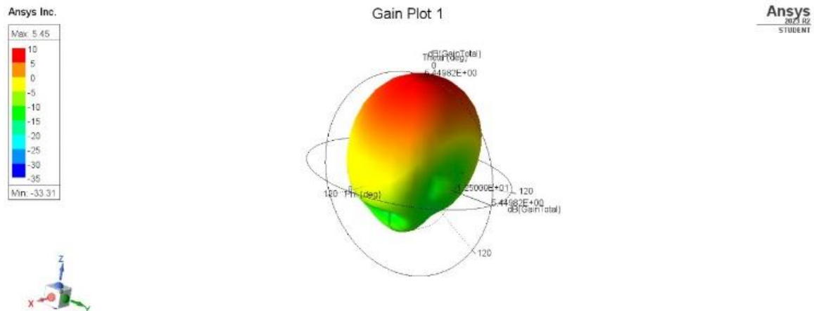
Figure 8. Antenna gain.
