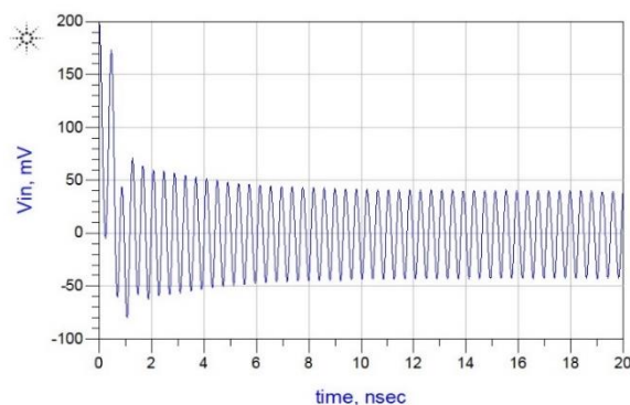
Figure 11. Vin (-10 dbm).
