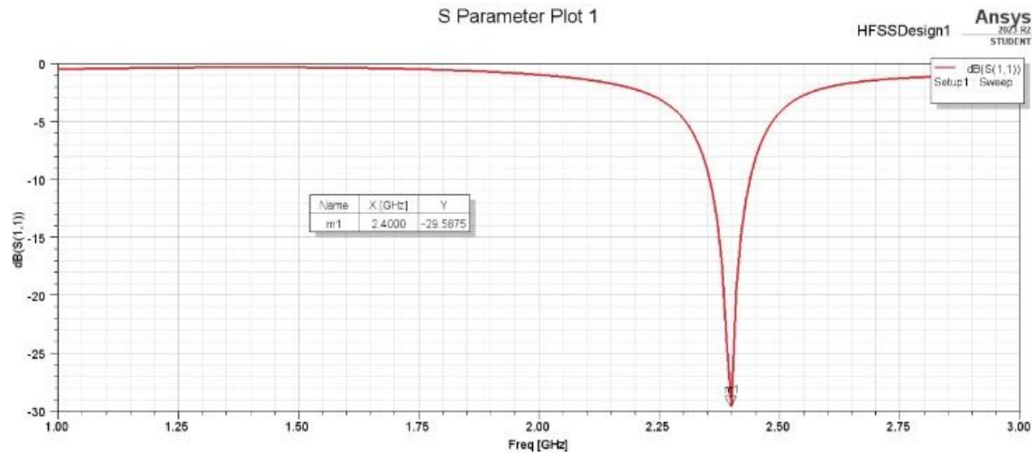
Figure 7. Antenna reflection coefficient.
