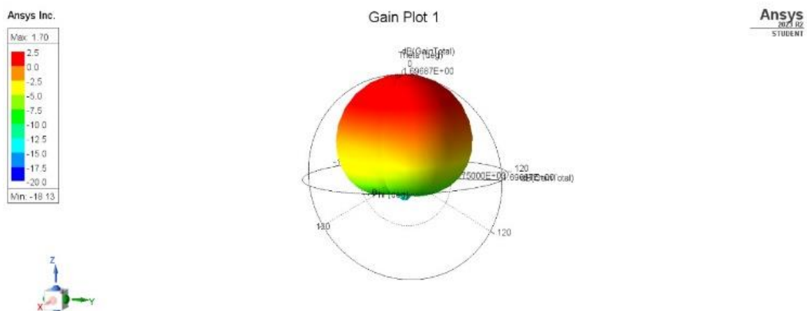
Figure 4. Antenna gain.
