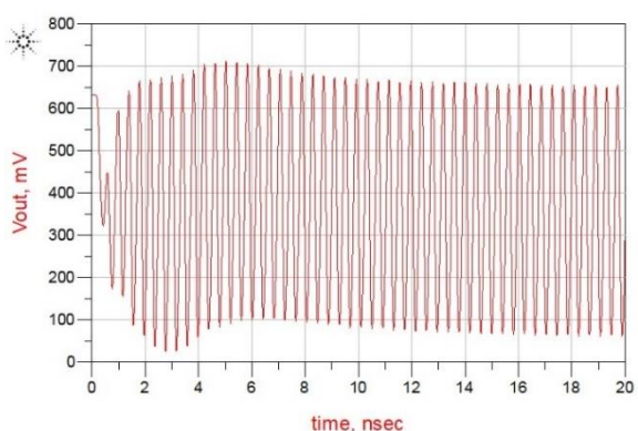
Figure 14. Vout at 0 dbm input power.
