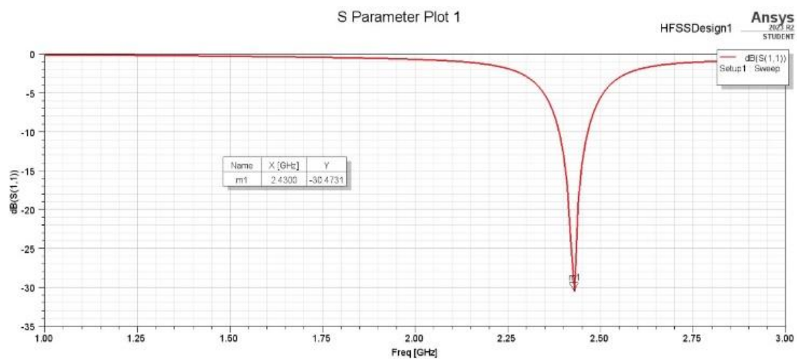
Figure 3. Antenna reflection coefficient.
