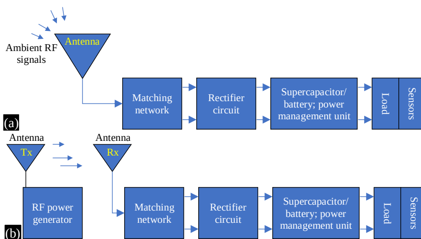
Figure 1. Block diagram of RF-EH system (a) RF energy harvesting, (b) Wireless power transfer.
