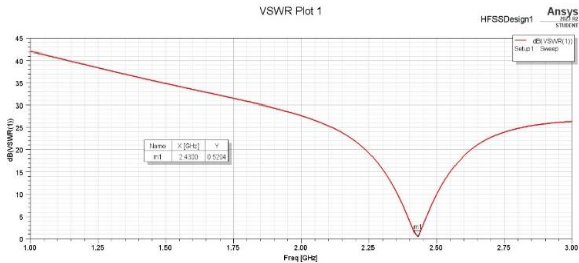
Figure 5. Antenna VSWR.
