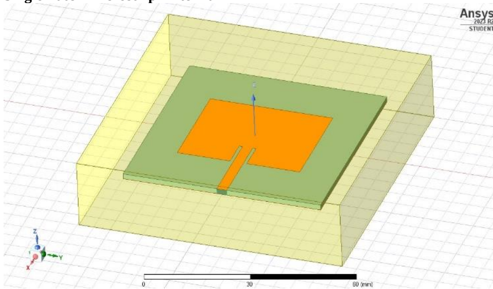
Figure 2. Single patch microstrip inset feed antenna in HFSS.
