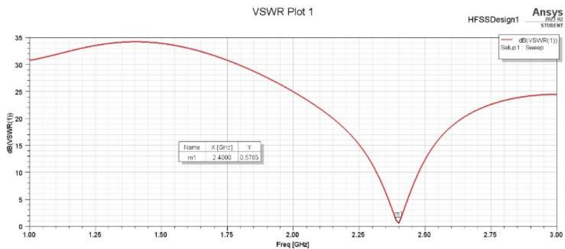
Figure 9. Antenna VSWR.
