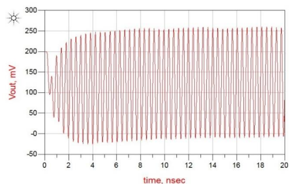
Figure 12. Vout at -10 dbm input power.
