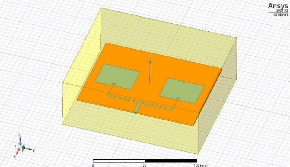
Figure 6: Dual patch microstrip inset feed antenna in HFSS.
