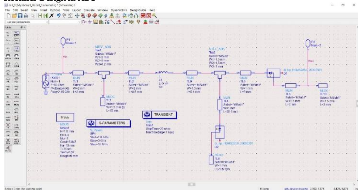
Figure 10. Rectifier in ADS.
