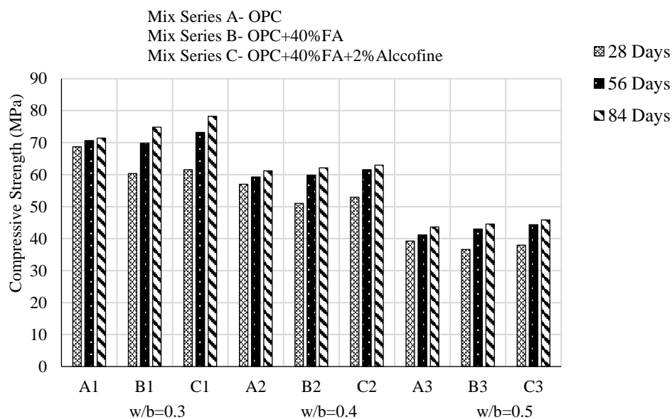
Figure 1. Compressive strength of concretes
