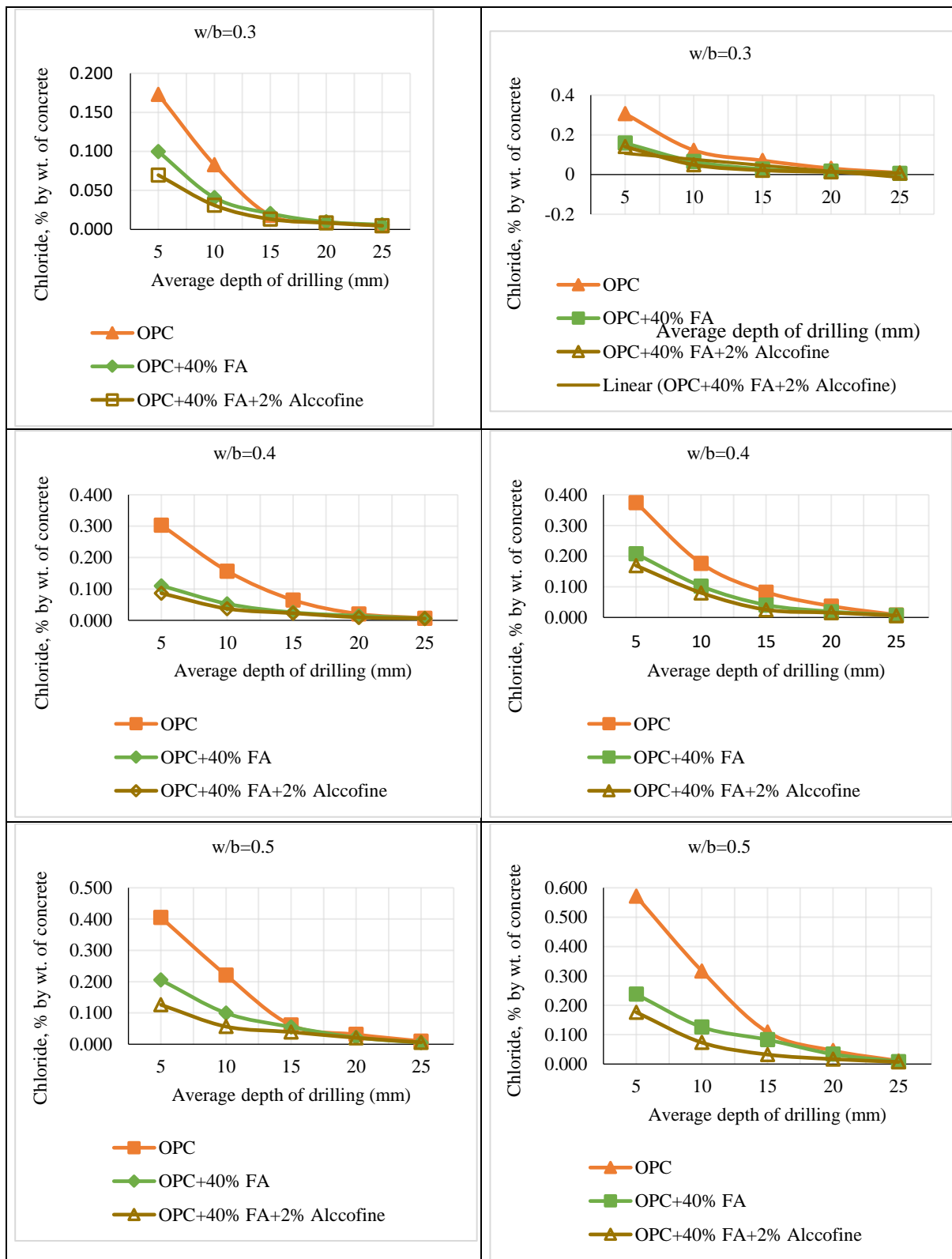
Figure 2. Chloride content at various depths
