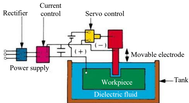
Figure 1. Electrical discharge machining.
