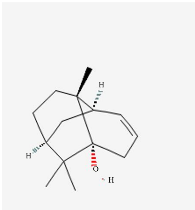
Figure 3. Norpatchoulenol.
