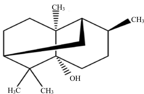
Figure 6. Patchoulol.
