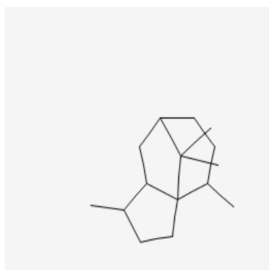
Figure 4. \beta -Patchoulene.
