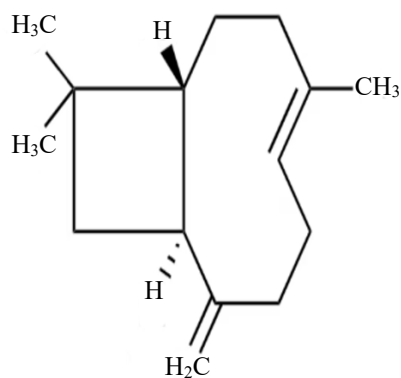
Figure 5. B-Caryophyllene.
