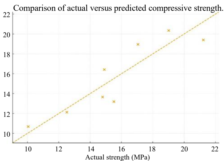
Figure 2. Predicted versus actual compressive strength.
