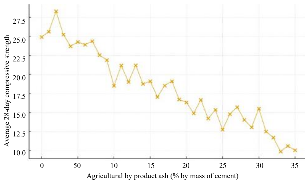
Variation of 28-day compressive strength with agricultural byproduct ash (ABA%)
