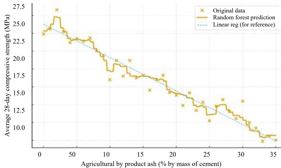
Figure 3. Random forest predicted curve across 0-35% ABA.
