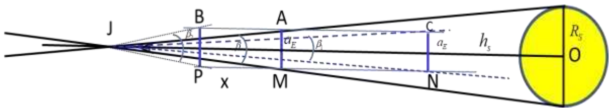
Figure 9. Showing how the Earth and the Sun can be observed as of equal size from point J in space. Length AM of the spherical cap base of the Earth visible from height h gets a single position between the Sun and the Earth, from where it subtends a visual angle \beta_s . For a position, say BP, its visual angle \beta_1 is greater, and for position CN, its visual angle \beta_2 is smaller than \beta_s .
