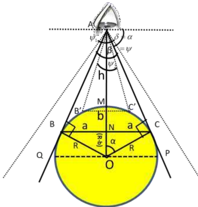
Figure 2. View of sphere of radius R as observed from height h . The spherical cap that is visible from point A with a view angle \psi = \beta is BMC , having height MN = b , tangent AC = AB represents the distance to the horizon, and NC = BN = a is the radius of the base of the visible spherical cap. For the relatively smaller angle of view \psi < \beta , a smaller spherical cap B'MC' can be seen, however, for the larger angle of view \psi > \beta , a larger visible spherical cap can be seen from the same height. The size perception for a large distance depends upon the visual angle \beta subtended at the eye of the observer.
