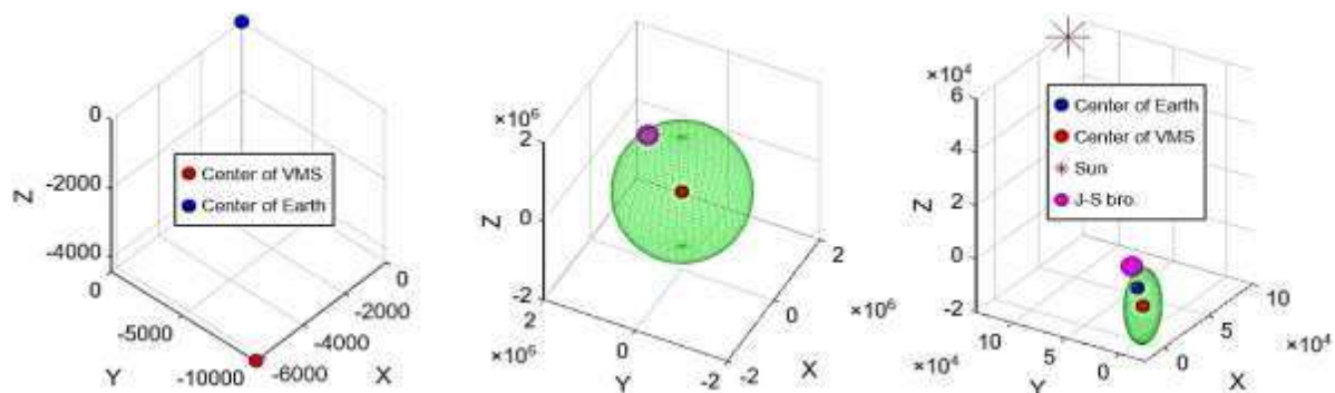
Figure 20. The first figure shows the estimated centers of MVS and CoE, the middle figure shows the spherical locus of J-S points on the Valmiki Sphere, and the rightmost figure shows all together with the Sun; however, the radius of MVS and the distance of the Sun have been scaled down by 100 and 50, respectively, to keep these things visible together.
