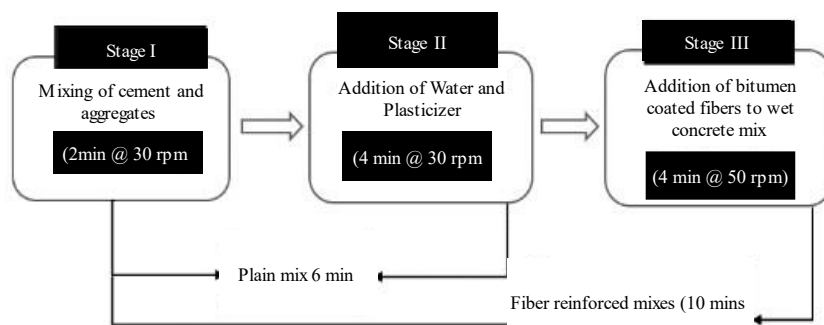
Figure 2. Phases of mixing was carried out to generate batches of concrete.
