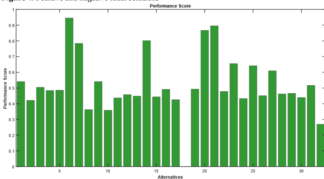
Figure 5. Performance score
