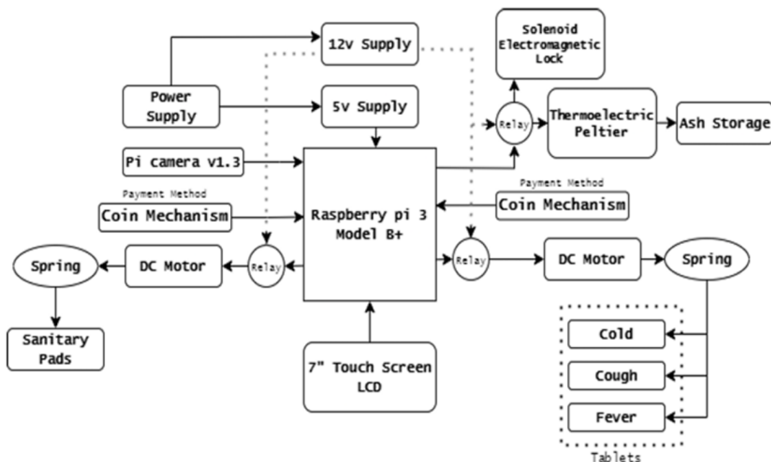
Figure 1 : Block Diagram of Medicine And Femmecare Sanitary Napkins Vending Machine
