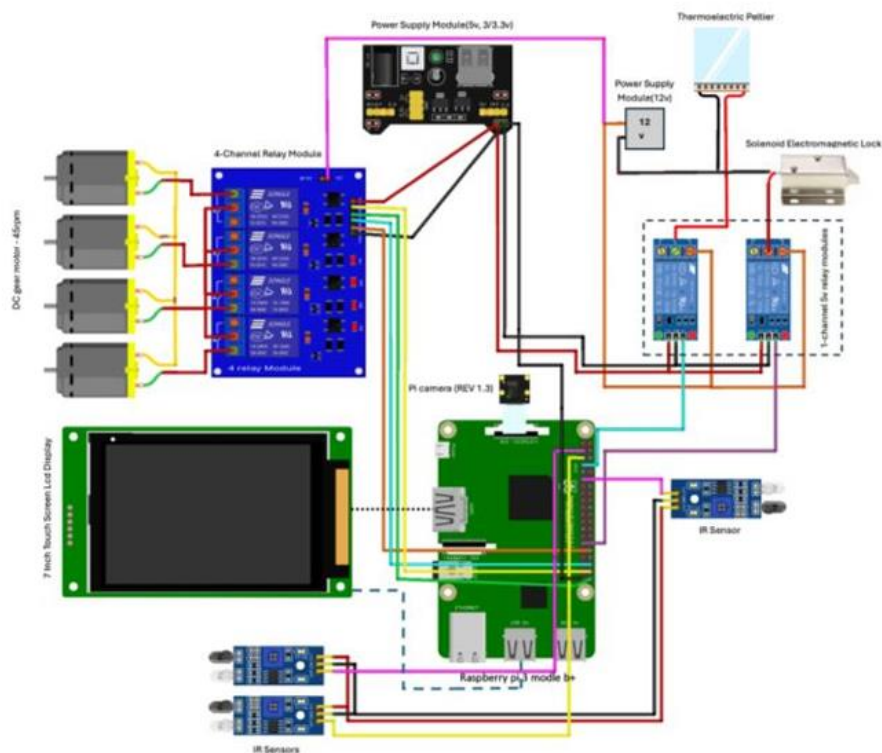
Figure 3: Technical Setup
