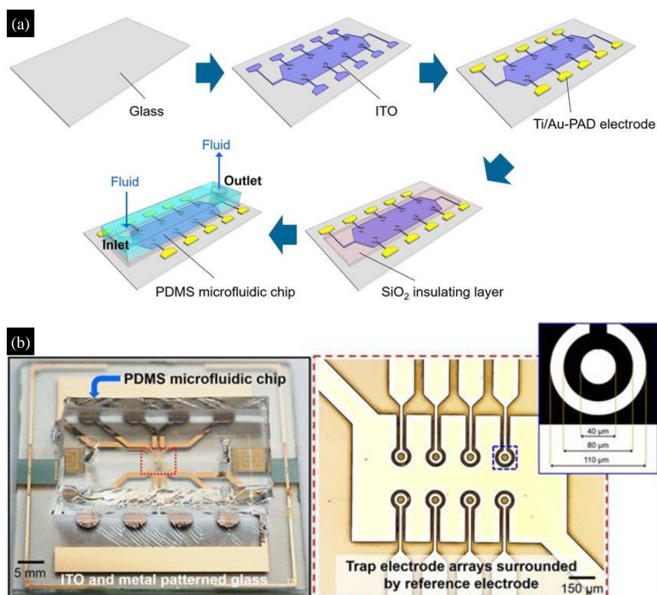
Figure 1. Microfluidic Device.
