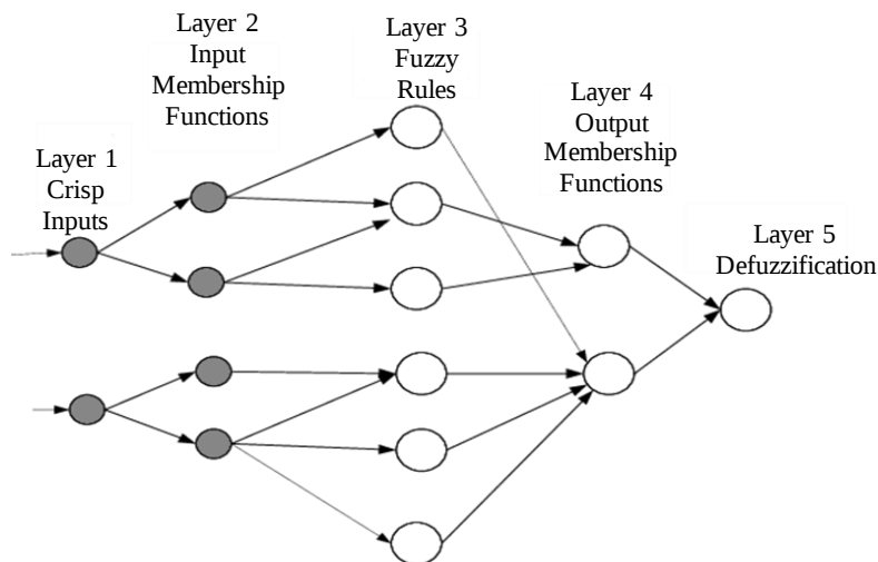
Figure 3. The five layer neuro-fuzzy structure.
