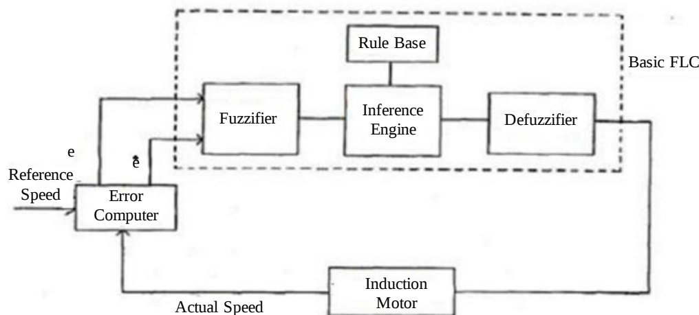
Figure 2. Block Configuration of Fuzzy Logic Controller
