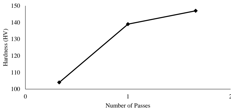
Figure 10. Vickers hardness of AA5083 before and after ECAP [23].
