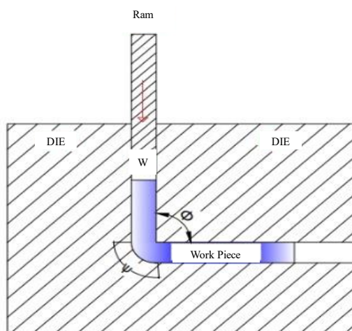
Figure 1. The schematic sketch of ECAP process [2].
