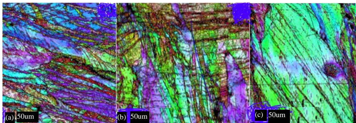
Figure 4. IPF map shows the state the application of the ECAP technique in the three planes of the ECAP billet, with high angle bounds ( > 15^\circ , red lines) and low angle boundaries ( > 2^\circ , black lines) for the three fundamental plane orientations [12].
