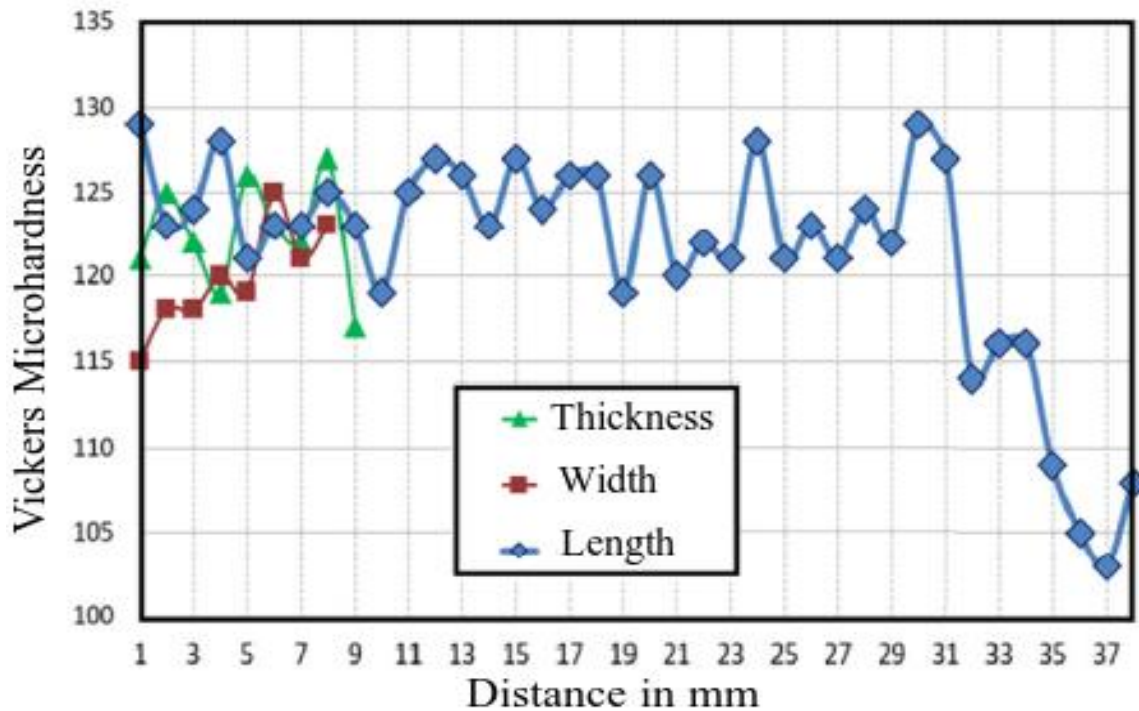
Figure 5. ECAP technique’s evaluation of the hardness values for the relevant directions and the Vickers microhardness profile measurement [13].
