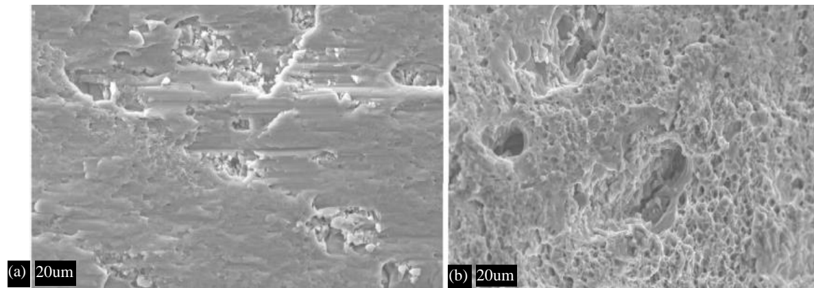
Figure 15. Typical fracture surface of AA5053 after ECAP in various tests: a) ST; b) MTT [31].
