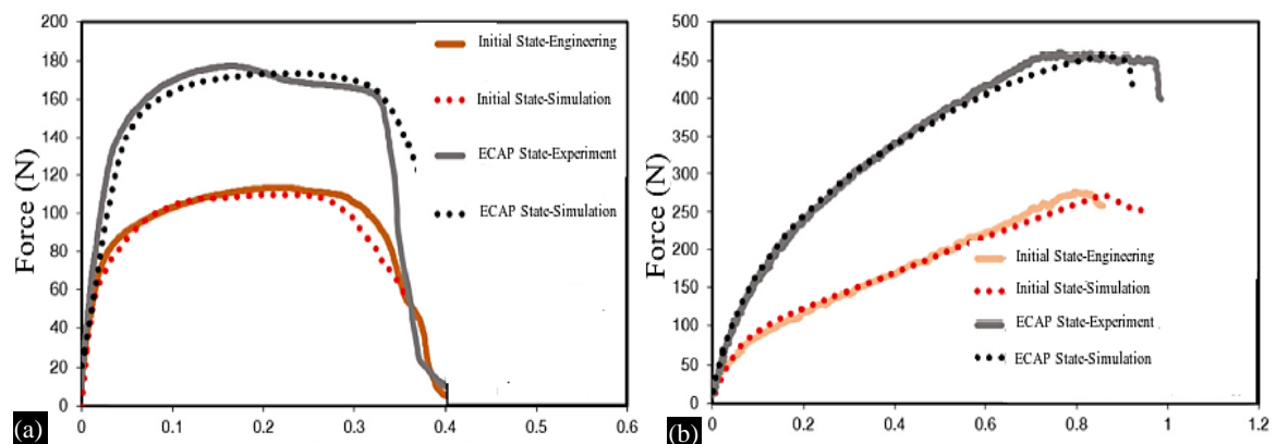
Figure 14. Test records for ST and BT specimen, including the results of the FEM simulation tests with damage [29], (a) Displacement (mm) ST (Vs) (b) Displacement (mm) BT
