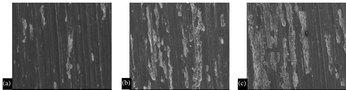
Figure 13. Wear on AA5083's surfaces as seen using SEM morphologies: (a) without ECAP; (b) after one pass; and (c) after two passes [27].
