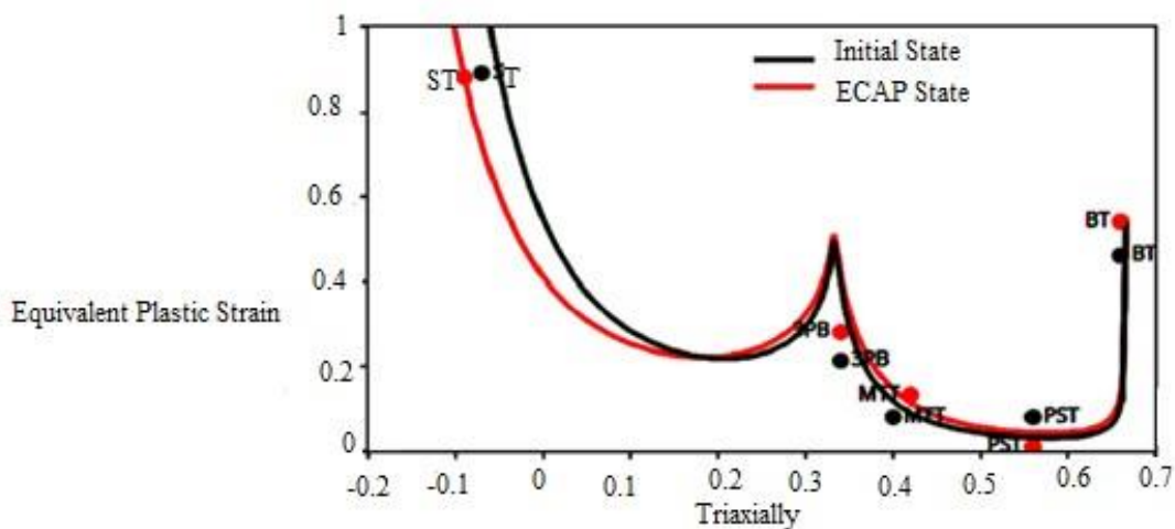
Figure 9. Fracture locus of Hosford–Coulomb model in two Dimensional [22].
