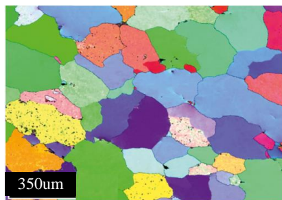
Figure 2. Microstructure of the AA5083 in the initial state [4].
