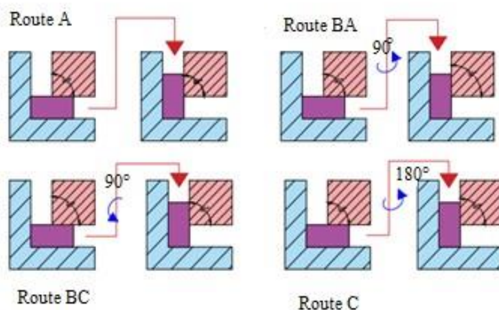
Figure 3. Procedure for different process of ECAP technique. [8]
