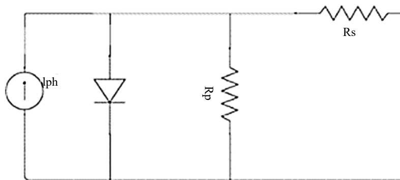
Figure 2. Standard equivalent circuit of a photovoltaic (PV) cell.
