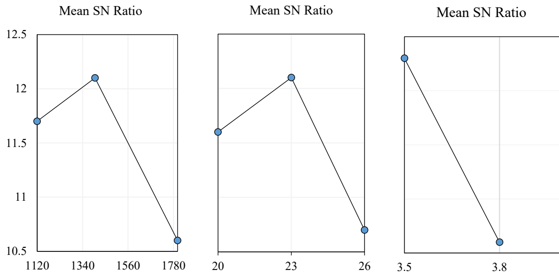
Figure 4. Effect of machining parameters on tensile for S/N ratio for larger is better.
