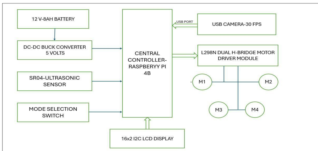
Figure 1: Block diagram of the ArUco marker guided smart trolley with integrated billing estimation
