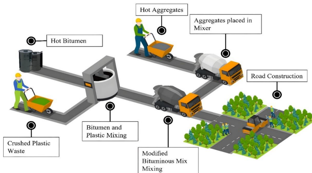
Figure 2. Wet process [3]
