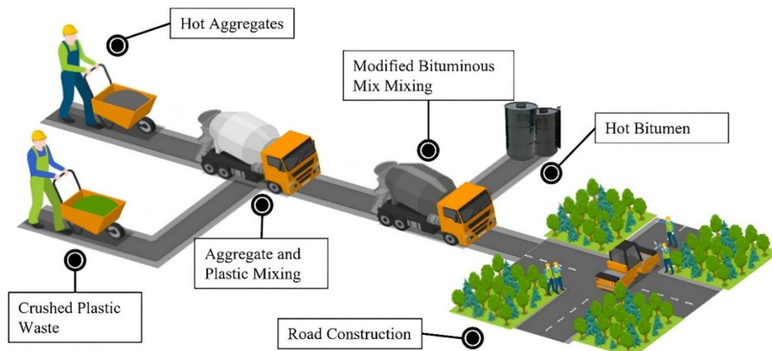
Figure 3. Dry process [3]
