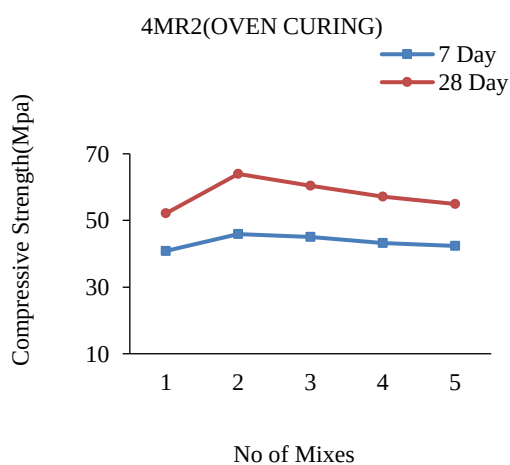
Figure 9. 4 Molar Ratio 2 oven drying values
