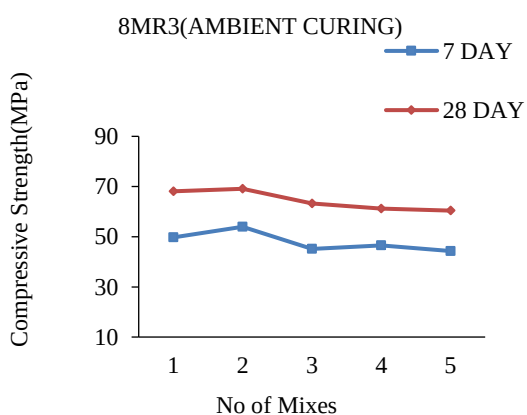
Figure 23. 8Molar R3 Ambient Curing
