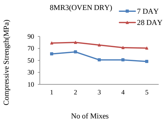
Figure 24. 8Molar R3 oven drying
