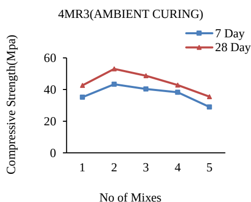
Figure 11. 4Molar Ratio 3 Ambient Curing
