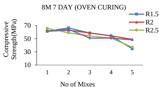
Figure 26. 8Molar 7day oven drying for all ratio's
