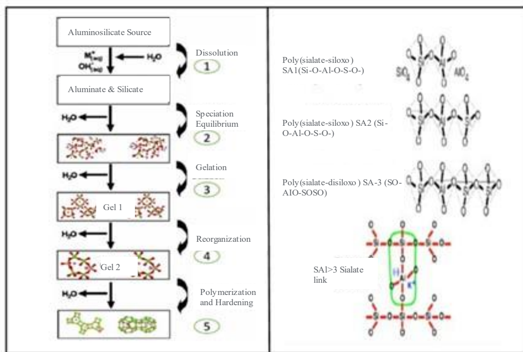
Figure 3. Process of geopolymerization
