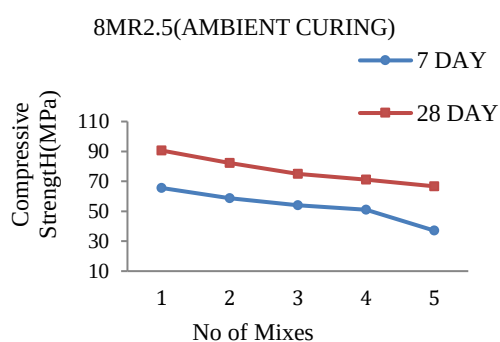
Figure 22. 8Molar R2.5 Ambient Curing
