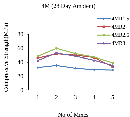
Figure 14. 4Molar 28day Ambient Curing for all ratio's
