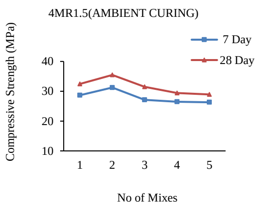
Figure 7. 4M R1.5 Ambient Curing
