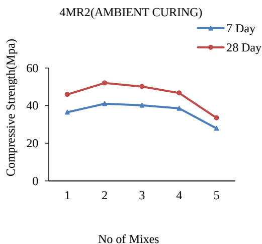
Figure 8. 4 Molar Ratio 2 Ambient Curing values
