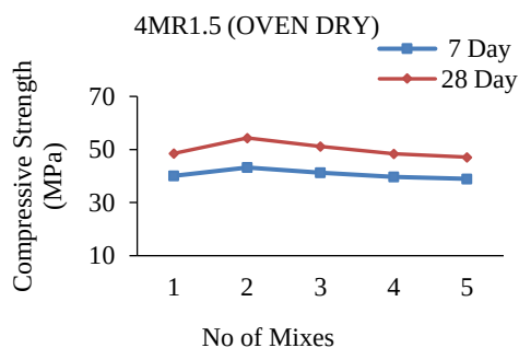
Figure 6. 4M R1.5 oven drying values
