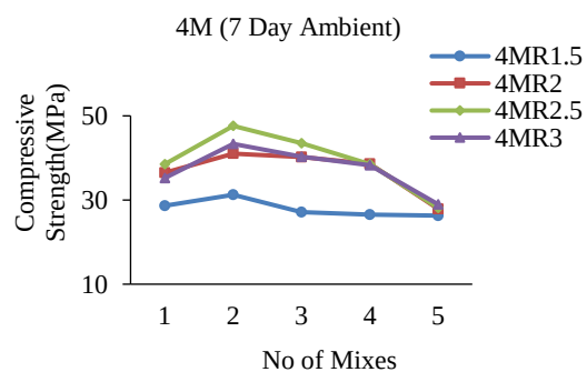
Figure 13. 4Molar 7-day Ambient Curing for all ratio's
