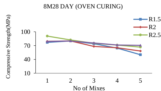
Figure 27. 8Molar 28day ambient drying for all ratio's
