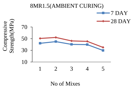
Figure 17. 8Molar R1.5 Ambient Curing
