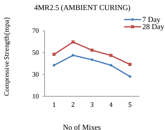
Figure 10. 4 Molar Ratio 2.5 Ambient Curing
