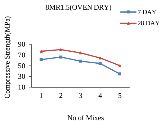
Figure 18. 8Molar R1.5 oven drying
