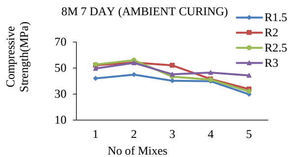
Figure 25. 8Molar 7day Ambient Curing for all ratio's
