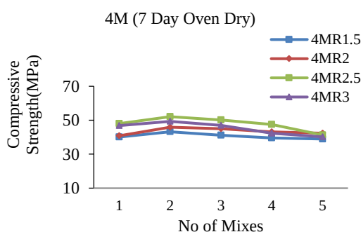
Figure 15. 4Molar 7day oven drying for all ratio's
