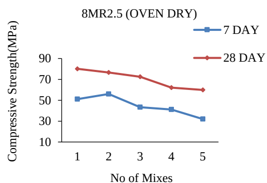
Figure 21. 8Molar R2.5 oven drying
