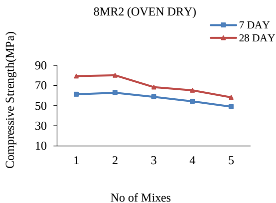
Figure 20. 8Molar R2 oven drying
