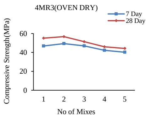
Figure 12. 4Molar Ratio 3 oven drying
