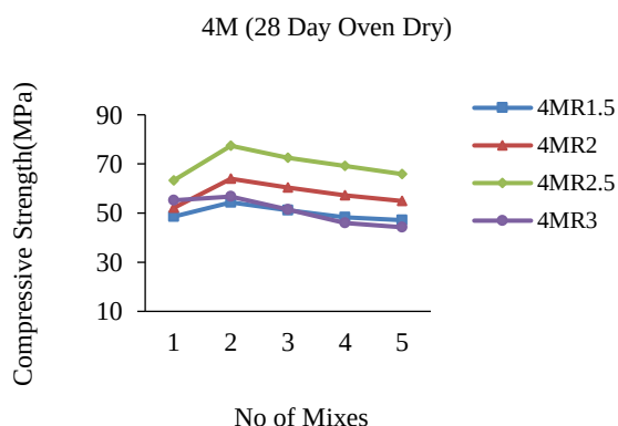
Figure 16. 4Molar 28day oven drying for all ratios
