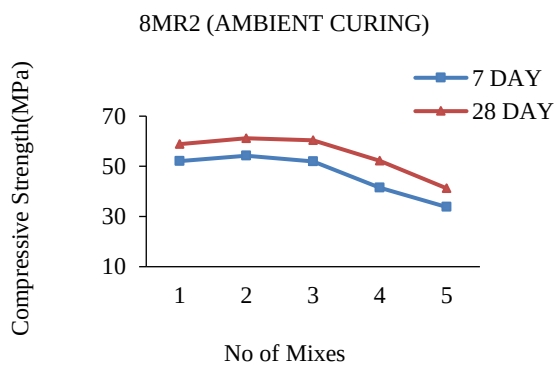
Figure 19. 8Molar R2 Ambient Curing
