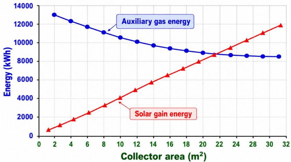
Figure 11. Solar and gas energy needs for air-cooling vs. collector area [55]
