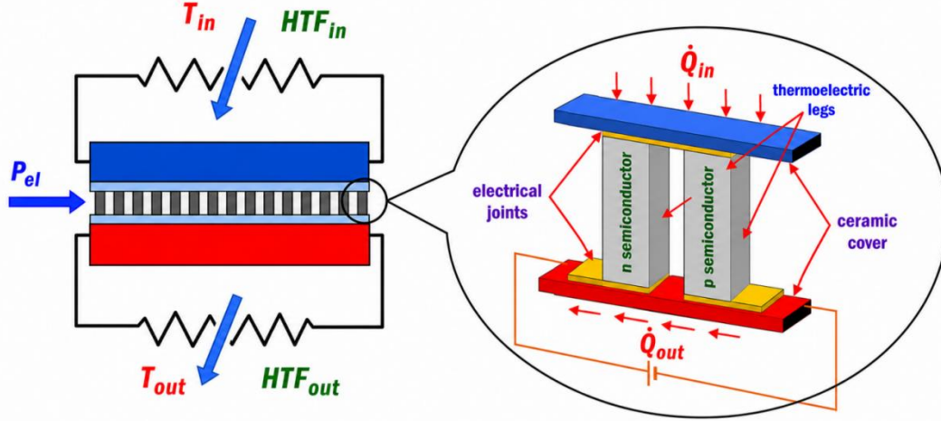
Figure 2. Schematic representation of the proposed air-conditioning system
