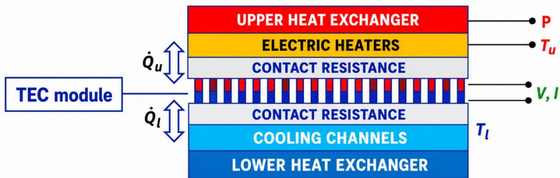
Figure 4. Schematic representation of the measurement system with an electrically heated upper heat exchanger at temperature T_u and a water-cooled lower heat exchanger at temperature T_l
