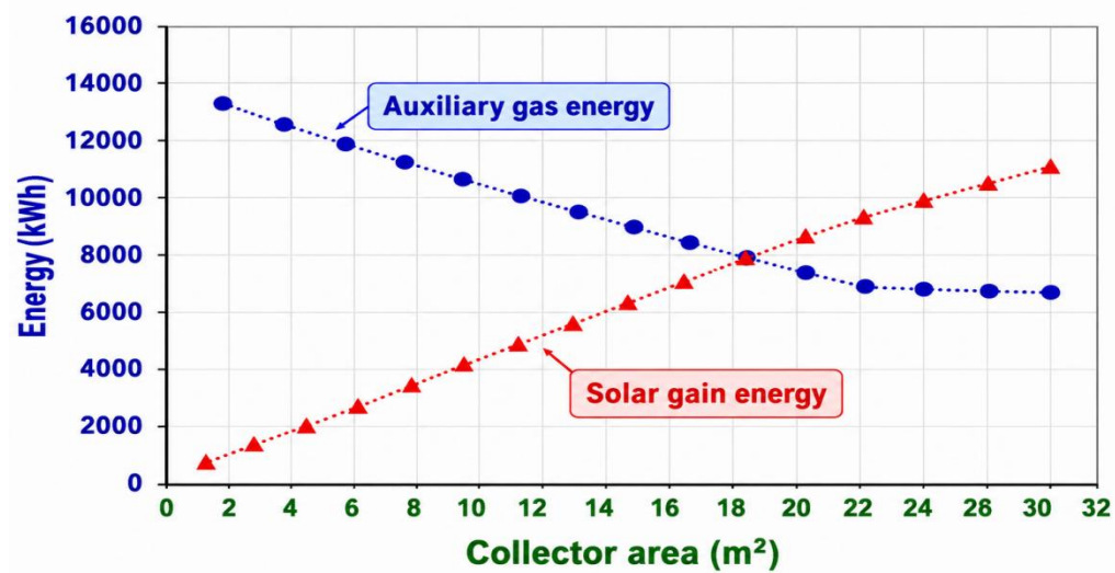
Figure 10. Solar and gas energy needs for water-cooling vs. collector area [54].
