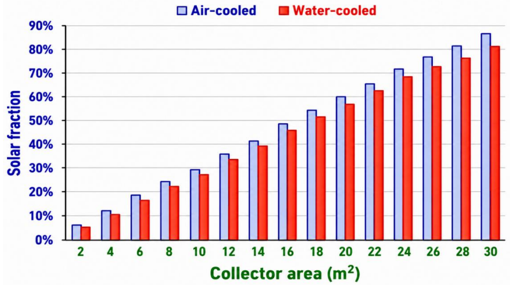
Figure 12. Solar fraction vs. collector area [56]
