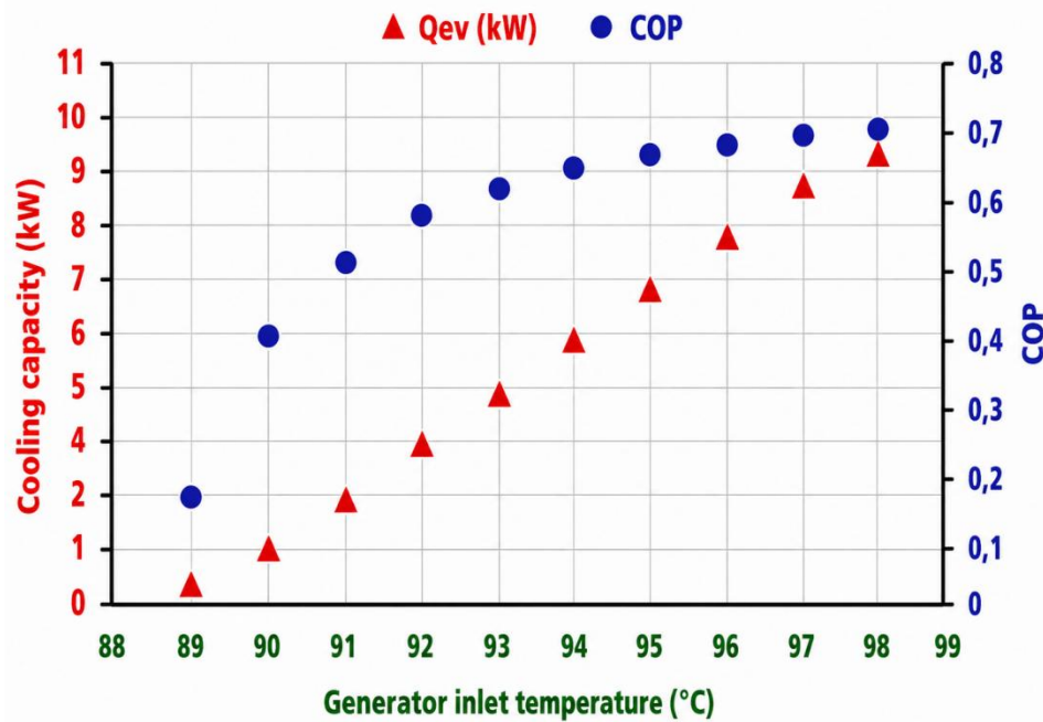
Figure 8. Effect of the generator inlet temperature on the performance of the absorption chiller [48].
