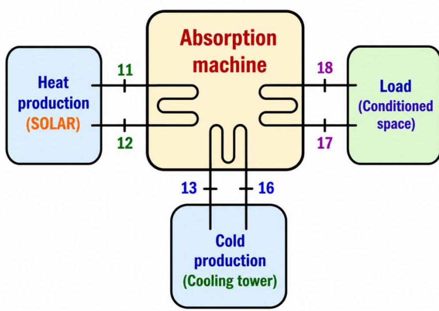
Figure 3. Schematic of unit's connections of solar assisted air-conditioning system [28].
