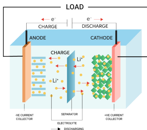
Figure 4. Lithium-ion battery
