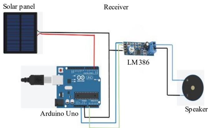
Figure 2. Block diagram of Receiver.
