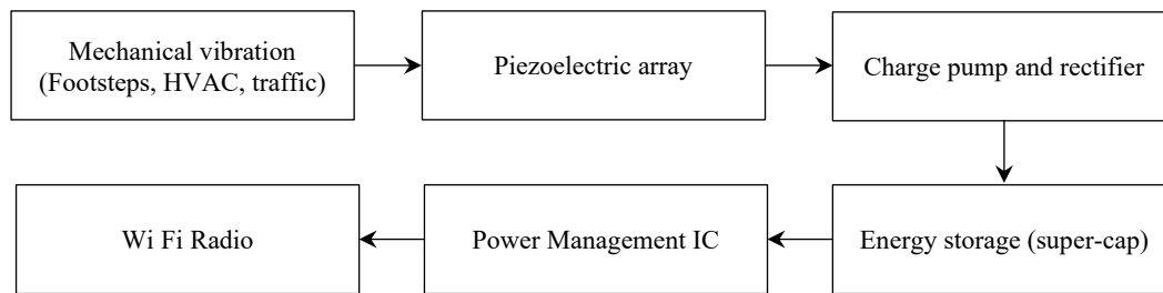
Figure 1. A high-level structure of a piezo-powered Wi-Fi node.
