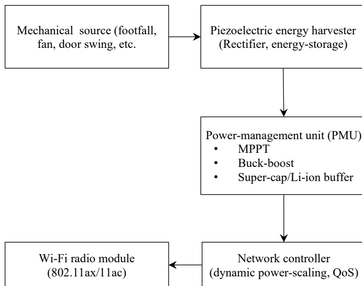
Figure 2. System-level architecture.
