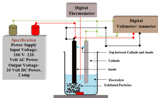
Fig: 1 Systematic diagram of exfoliation process of graphite
