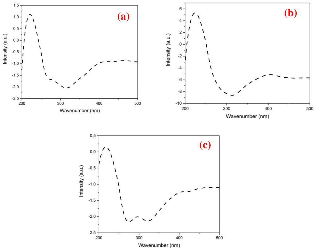
Fig: 7 UV-visible spectra of a) TrGO-650°C b) TrGO-750°C c) TrGO-850°C
