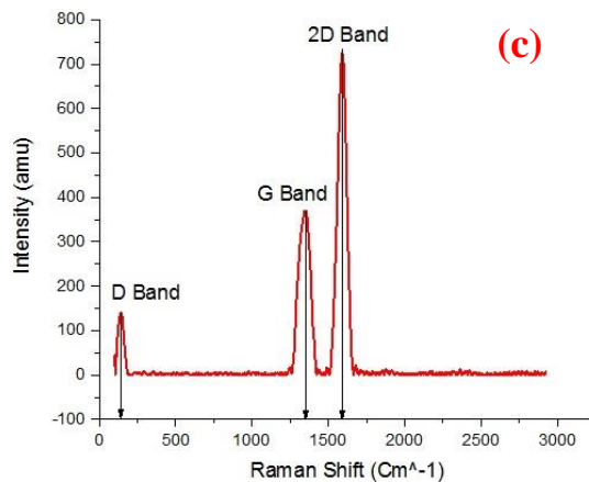
Fig: 5 Raman spectra identified for a) TrGO-650°C b) TrGO-750°C c) TrGO-850°C
