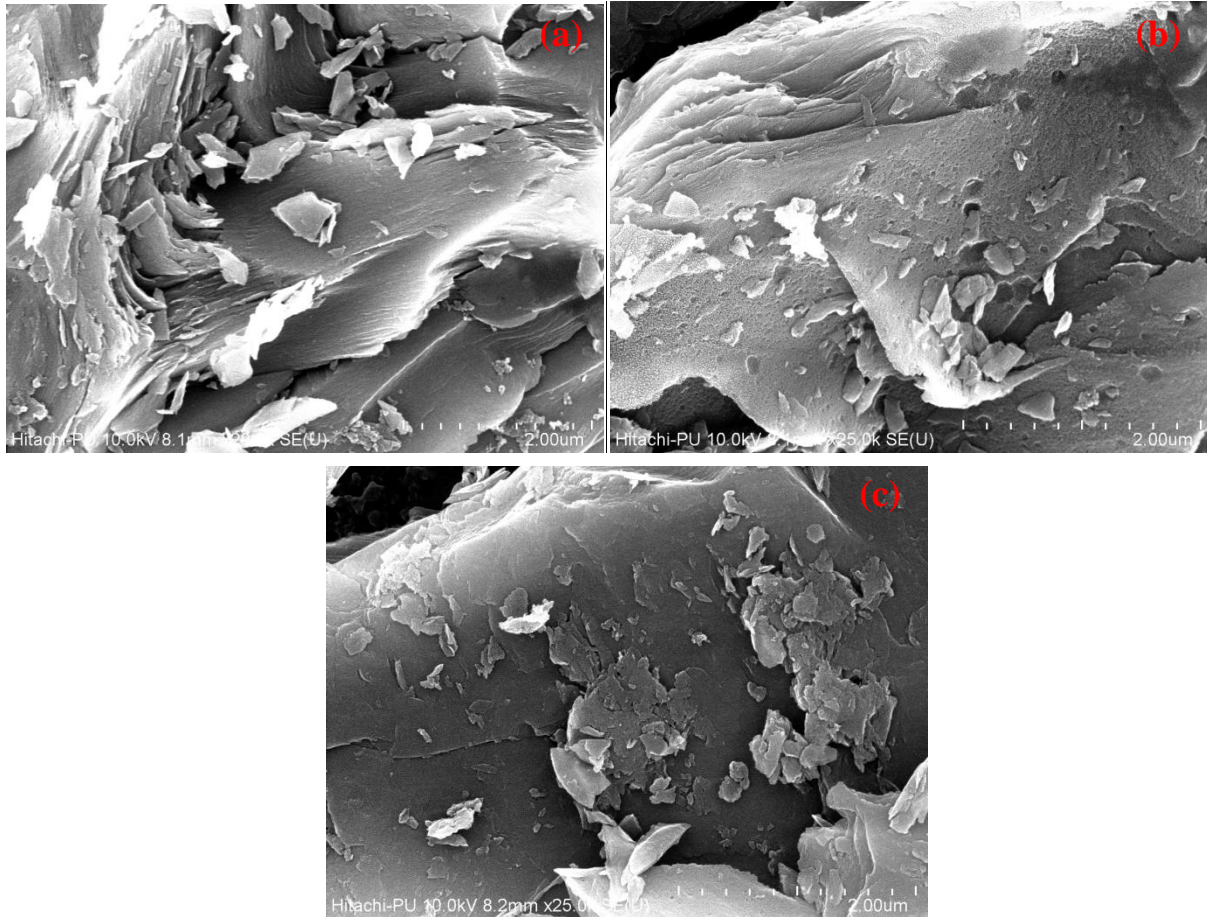
Fig: 4 FESEM with EDS images of a) TrGO-650°C b) TrGO-750°C c) TrGO-850°C at 2 μm
