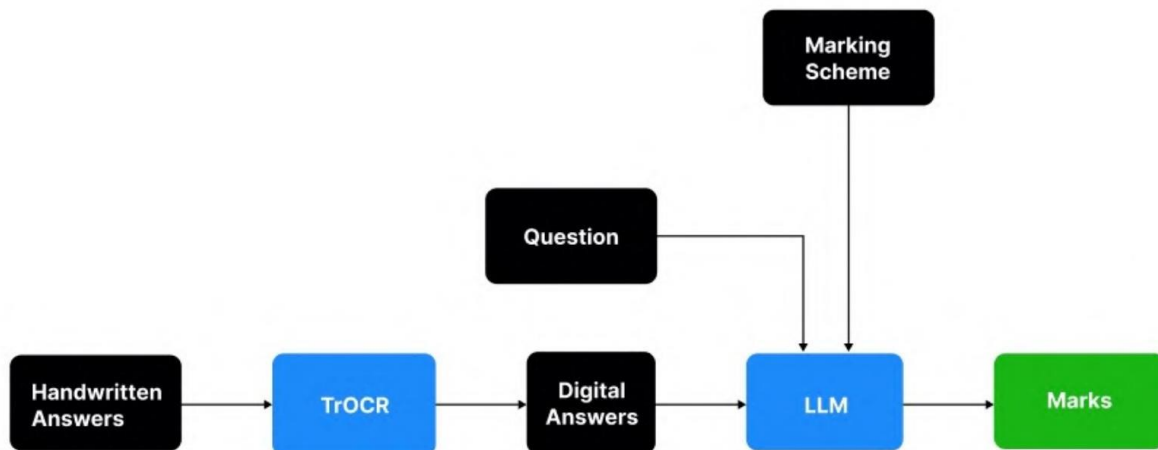
Figure-1. Flowchart of AI Evaluator
