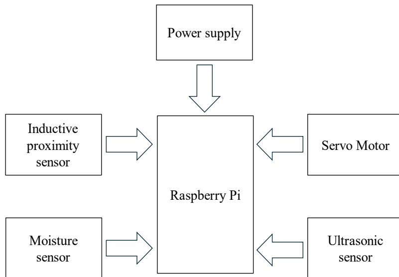
Figure 8. System Design.
