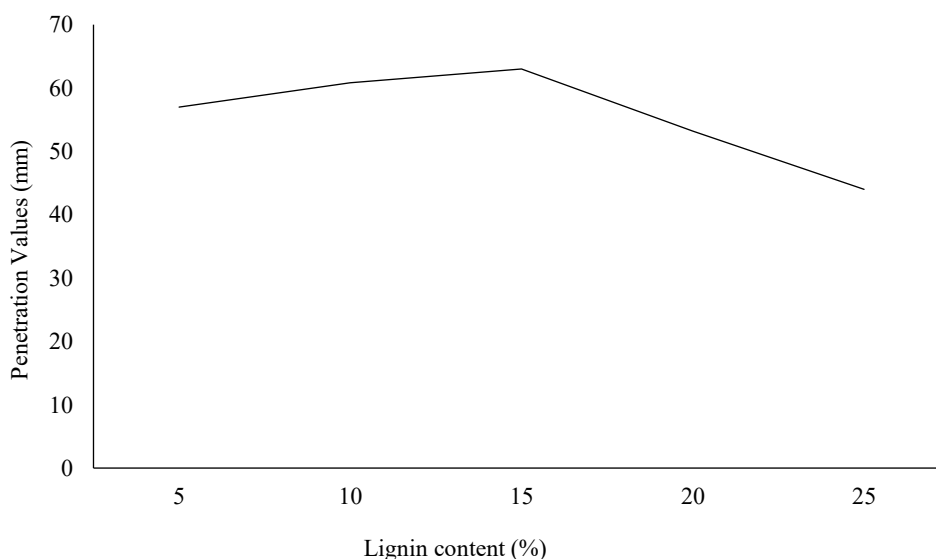
Figure 3. Graph showing variation in penetration values.
