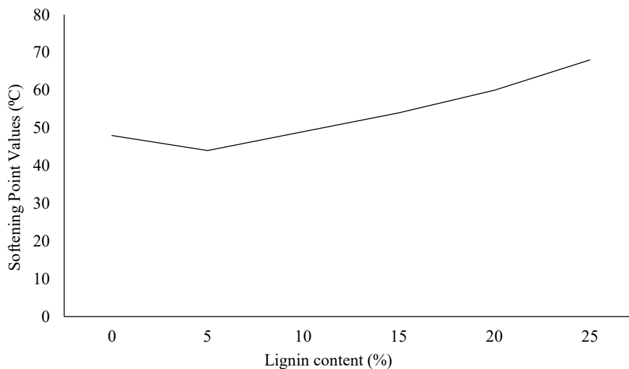
Figure 4. Graph showing variation in softening point values.
