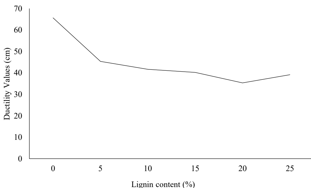
Figure 2. Graph showing variation in ductility values.
