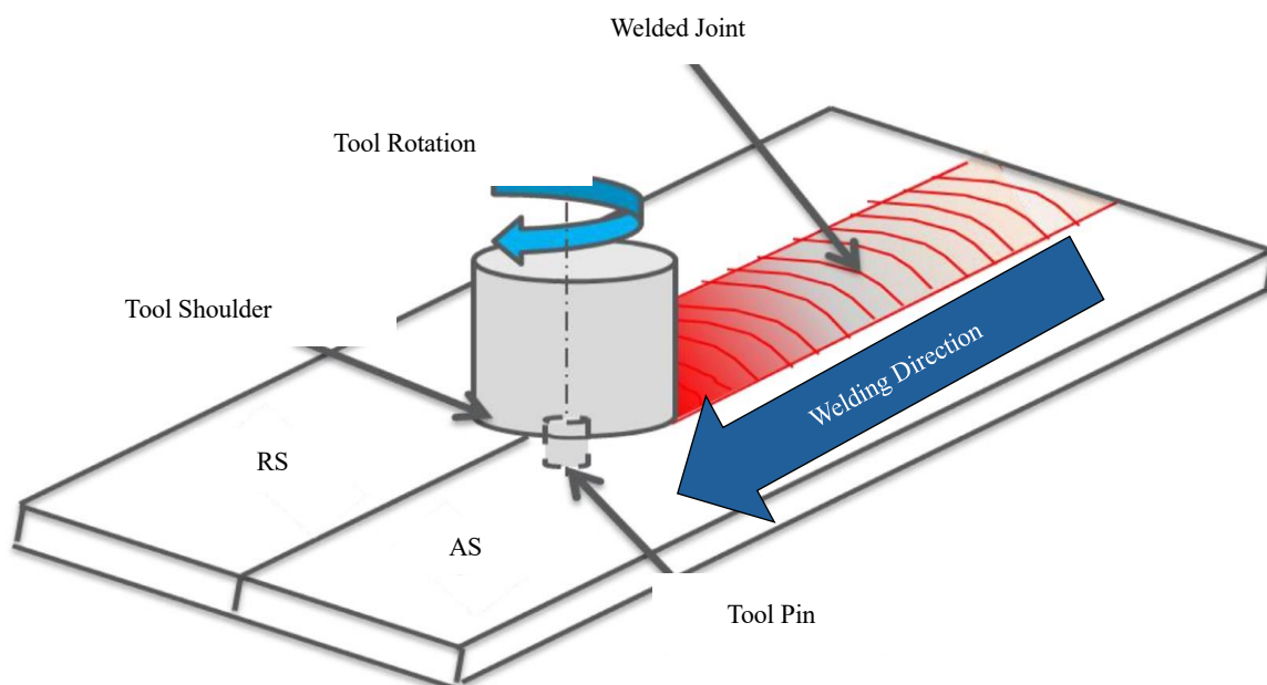
Figure 1. Diagrammatic illustration of the FSW procedure [10].
