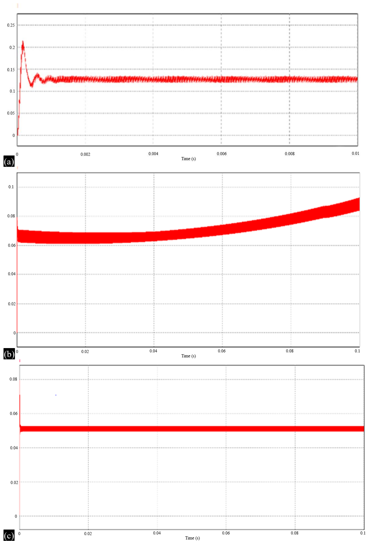
Figure 6. Output current for switching modes (a) Gate pulse (b) Square wave (c) PWM input
