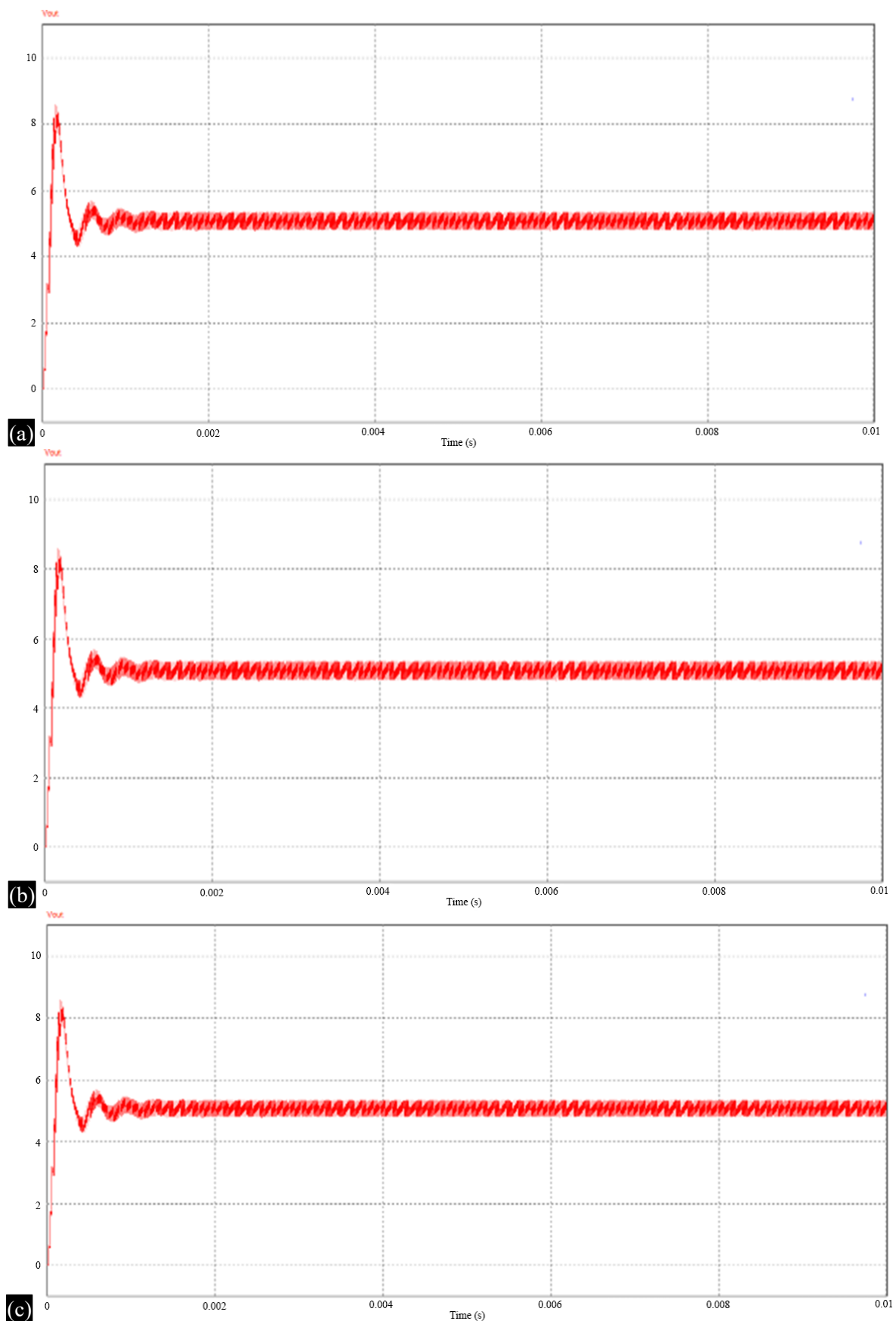
Figure 5. Output voltage for switching modes (a) Gate pulse (b) Square wave (c) PWM input
