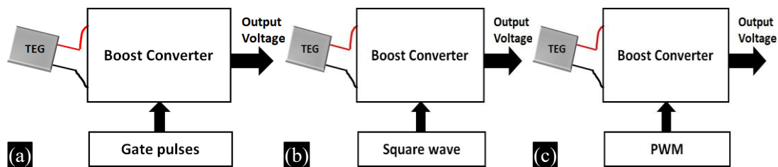
Figure 3. Block diagram of boost circuit with different switching sources (a) Gate switching (b) Square wave switching (c) PWM switching
