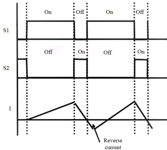
Figure 2. Inductor current in CCM
