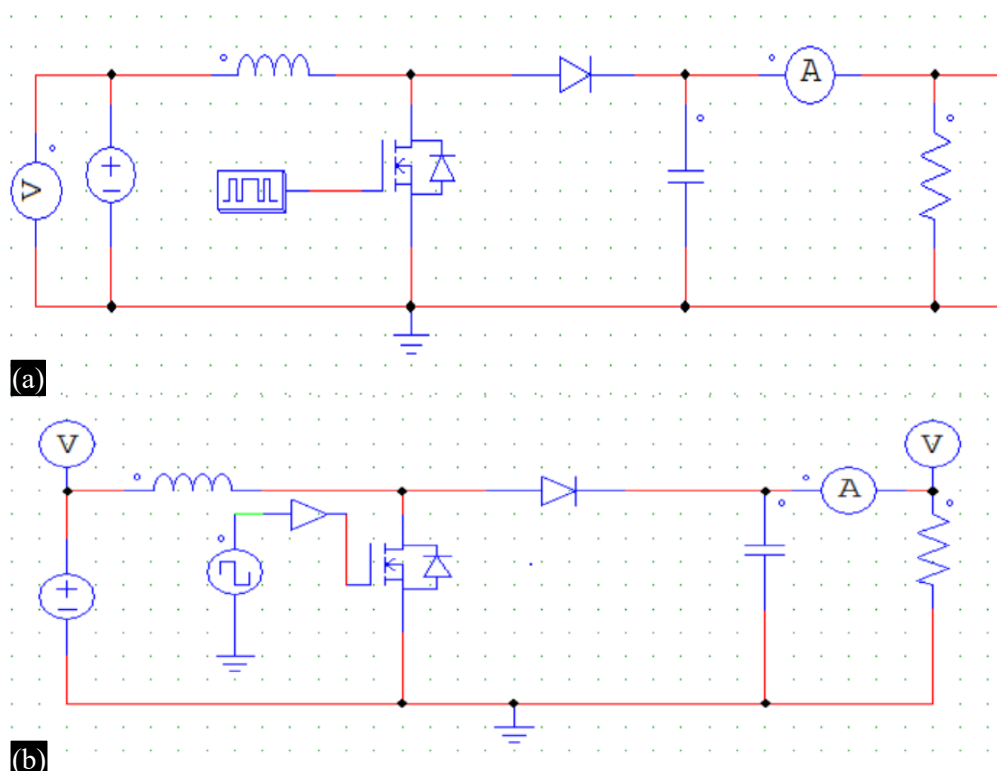
Figure 3. Block diagram of boost circuit with different switching sources (a) Gate switching (b) Square wave switching (c) PWM switching
