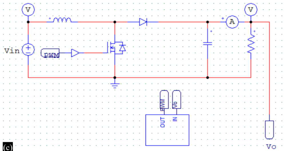
Figure 4. PSIM models of boost converter (a) Gate pulse control (b) Square wave control (c) PWM control boost circuit
