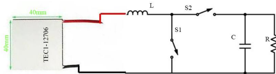
Figure 1. Basic Boost Converter.
