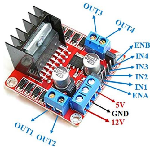
Figure 5. LN298N Motor Driver.
