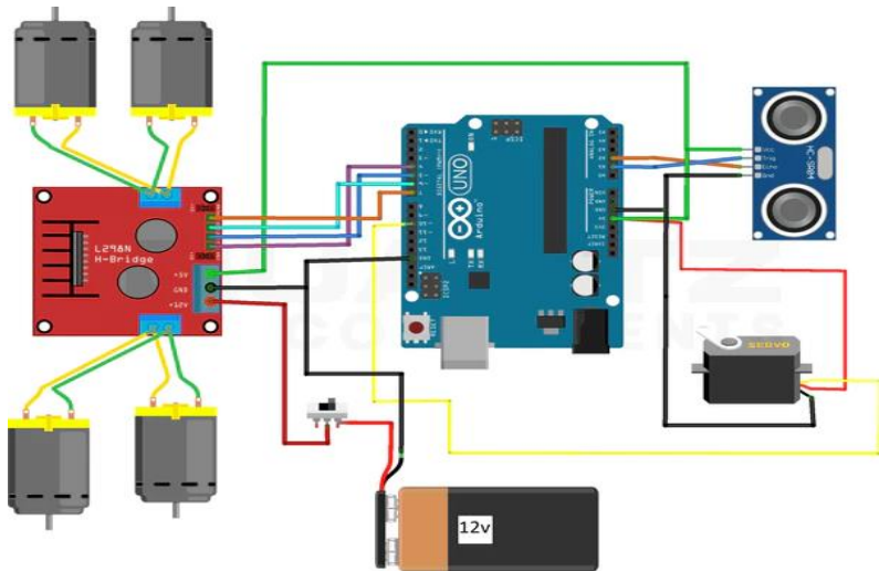
Figure 8. Circuit Diagram.
