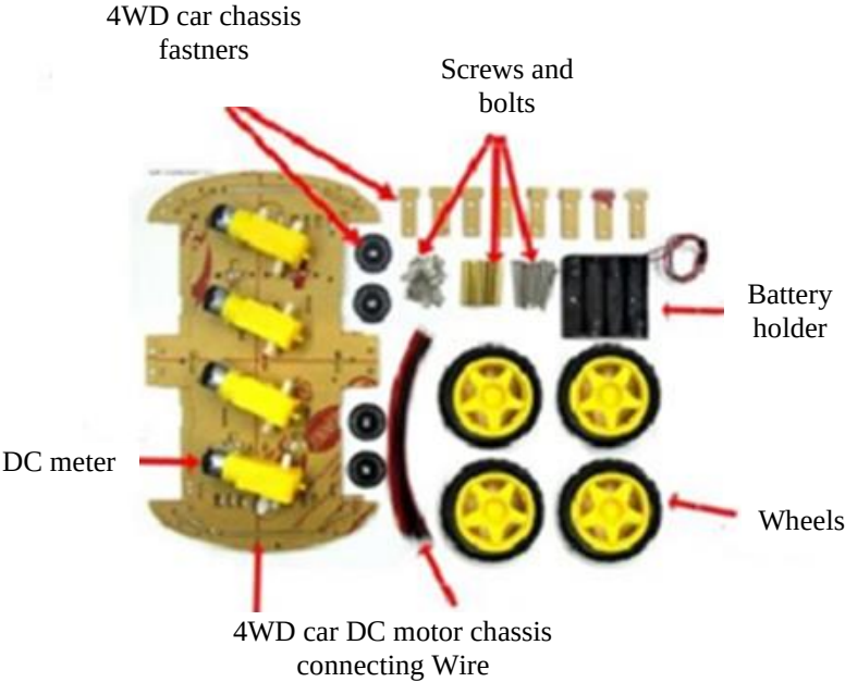
Figure 7. Robot Chassis.
