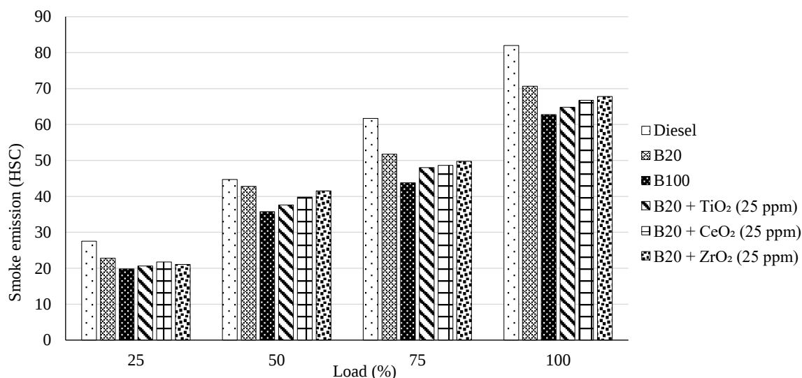
Figure 8. Smoke opacity Vs Load.
