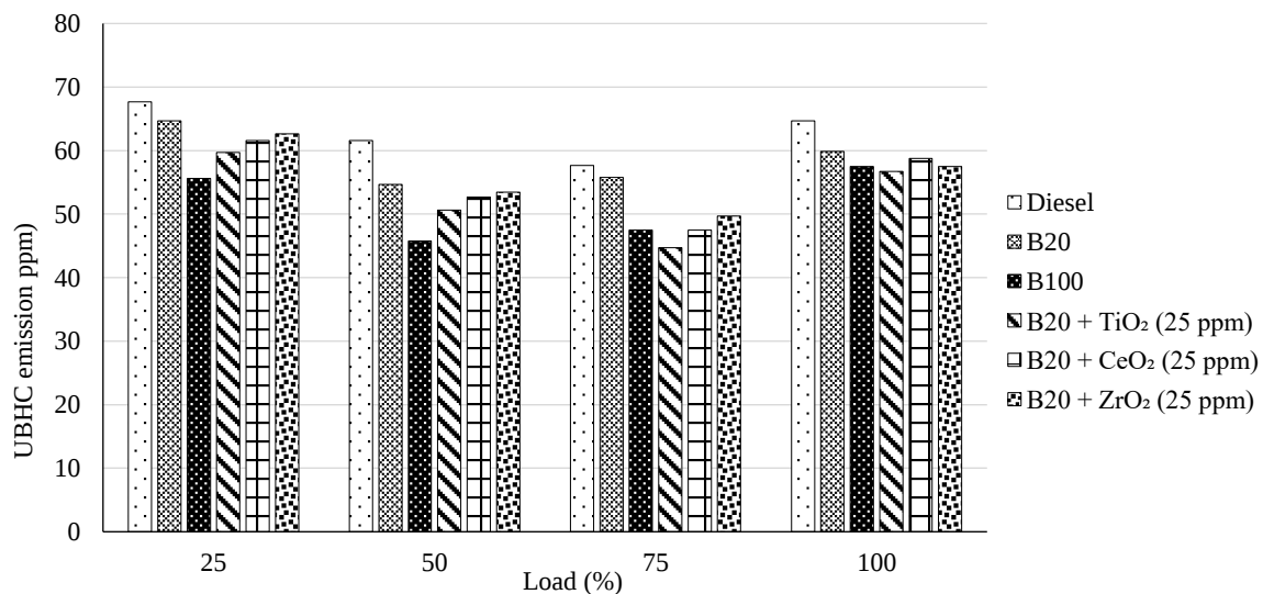
Figure 6. Unburnt hydrocarbon Vs Load.
