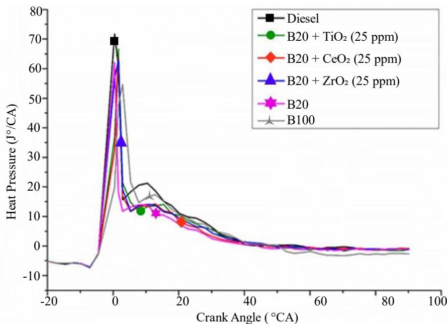
Figure 10. Heat Release Rate Vs Crank angle.
