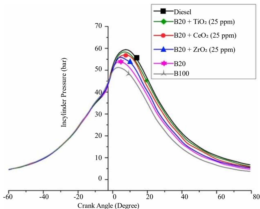
Figure 9. Cylinder pressure Vs Crank angle.
