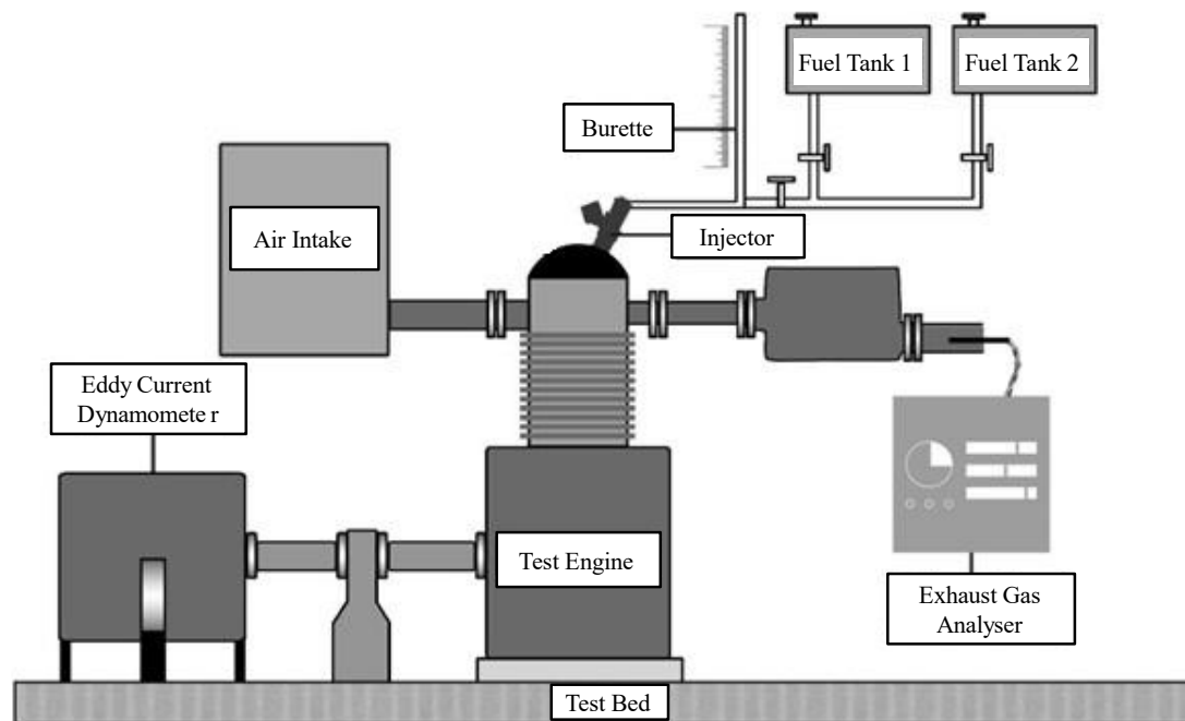
Figure 2. Engine set up.
