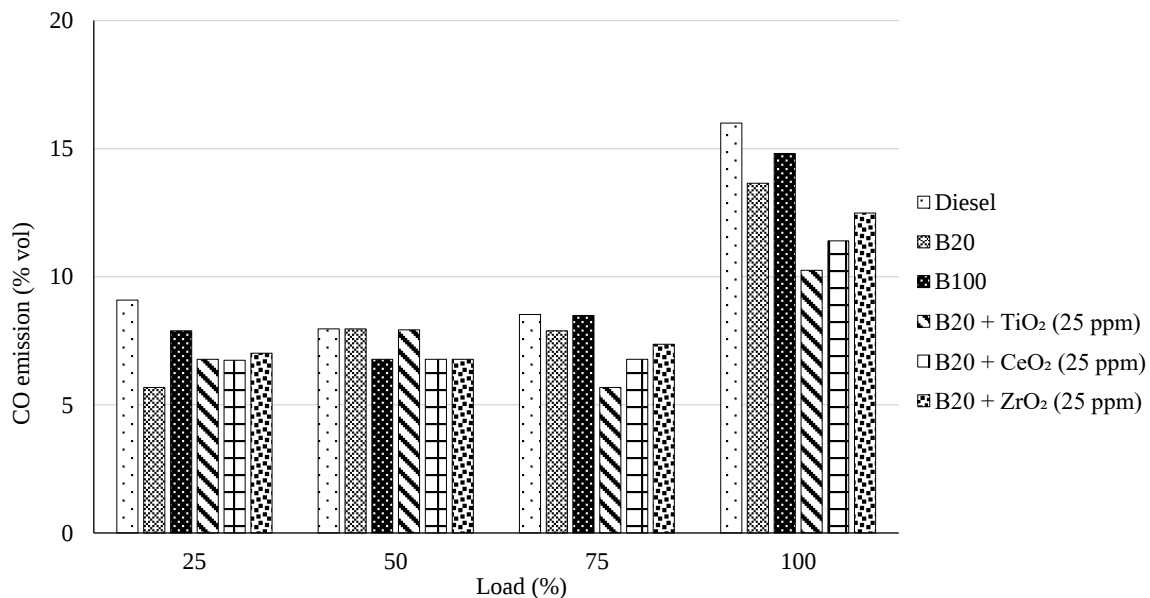
Figure 5. CO Emission Vs Load.
