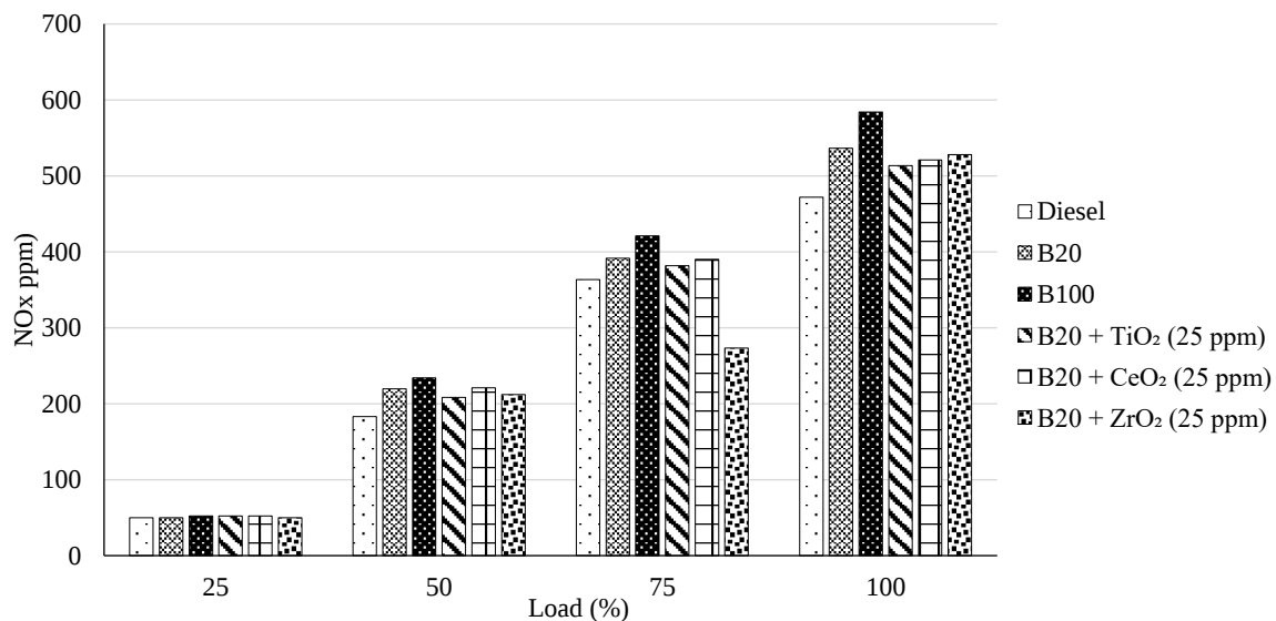
Figure 7. Oxides of nitrogen Vs Load.
