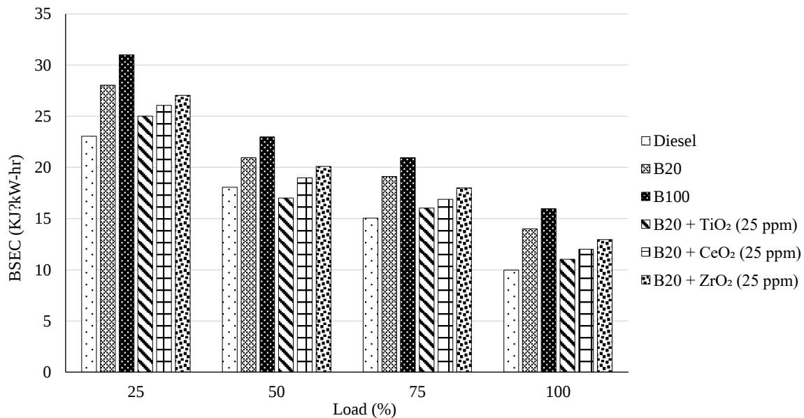
Figure 4. Specific fuel energy consumption Vs Load.
