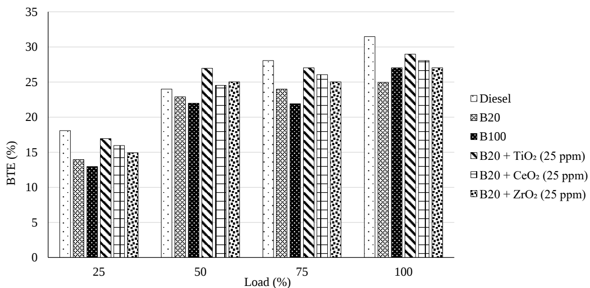
Figure 3. Brake thermal efficiency Vs Load.
