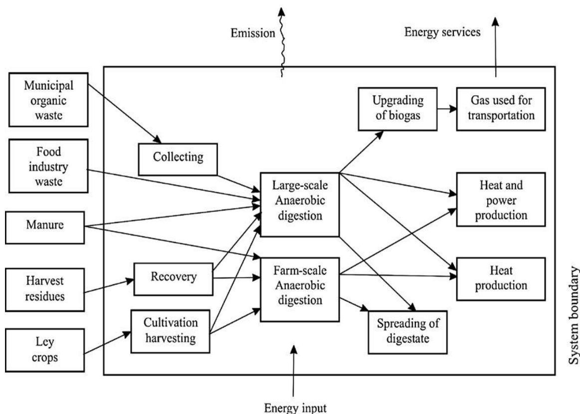
Figure 3. Overview of the examined biogas systems. The system's material, energy, and emission flows are depicted by arrows.
