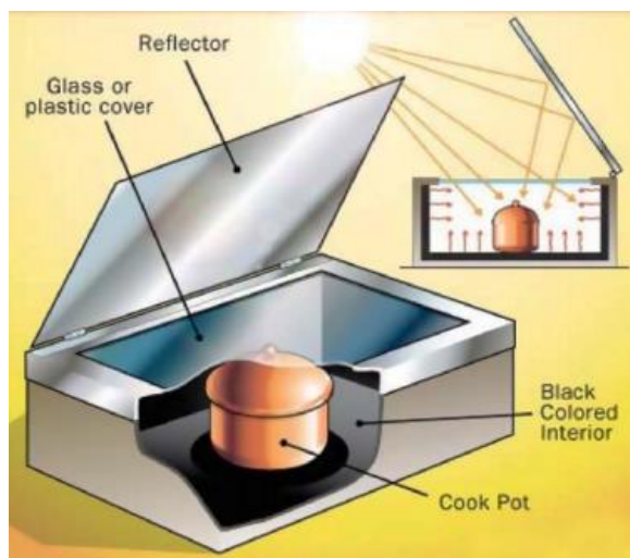
Figure 1. Solar-powered box cooker.
