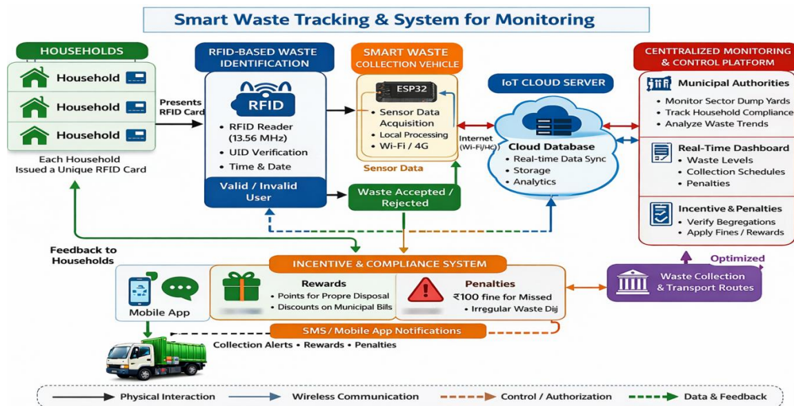
Figure 1. Block diagram of the proposed smart waste tracking and monitoring system
