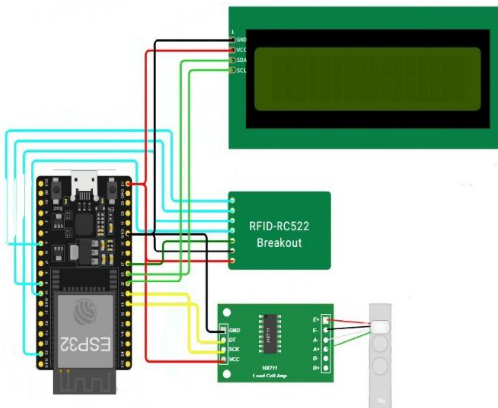
Figure 3. Circuit Diagram of the Dumping Yard Module
