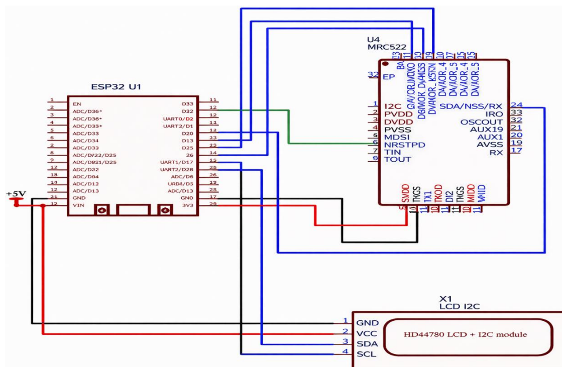
Figure 2. Circuit diagram of the Garbage Collection Vehicle Module
