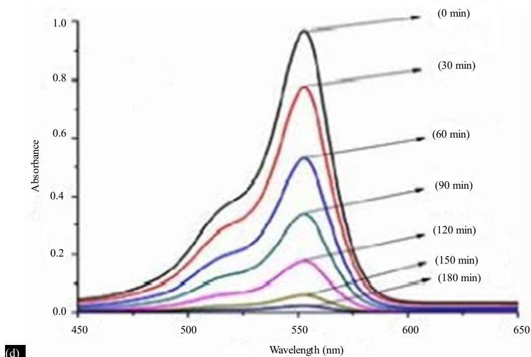
Figure 2. Absorbance spectral variations of blue -Methylene & Brhodamine by means of Cobalt Sulfide in Figure 1.c & 1.d underneath ultraviolet light.
