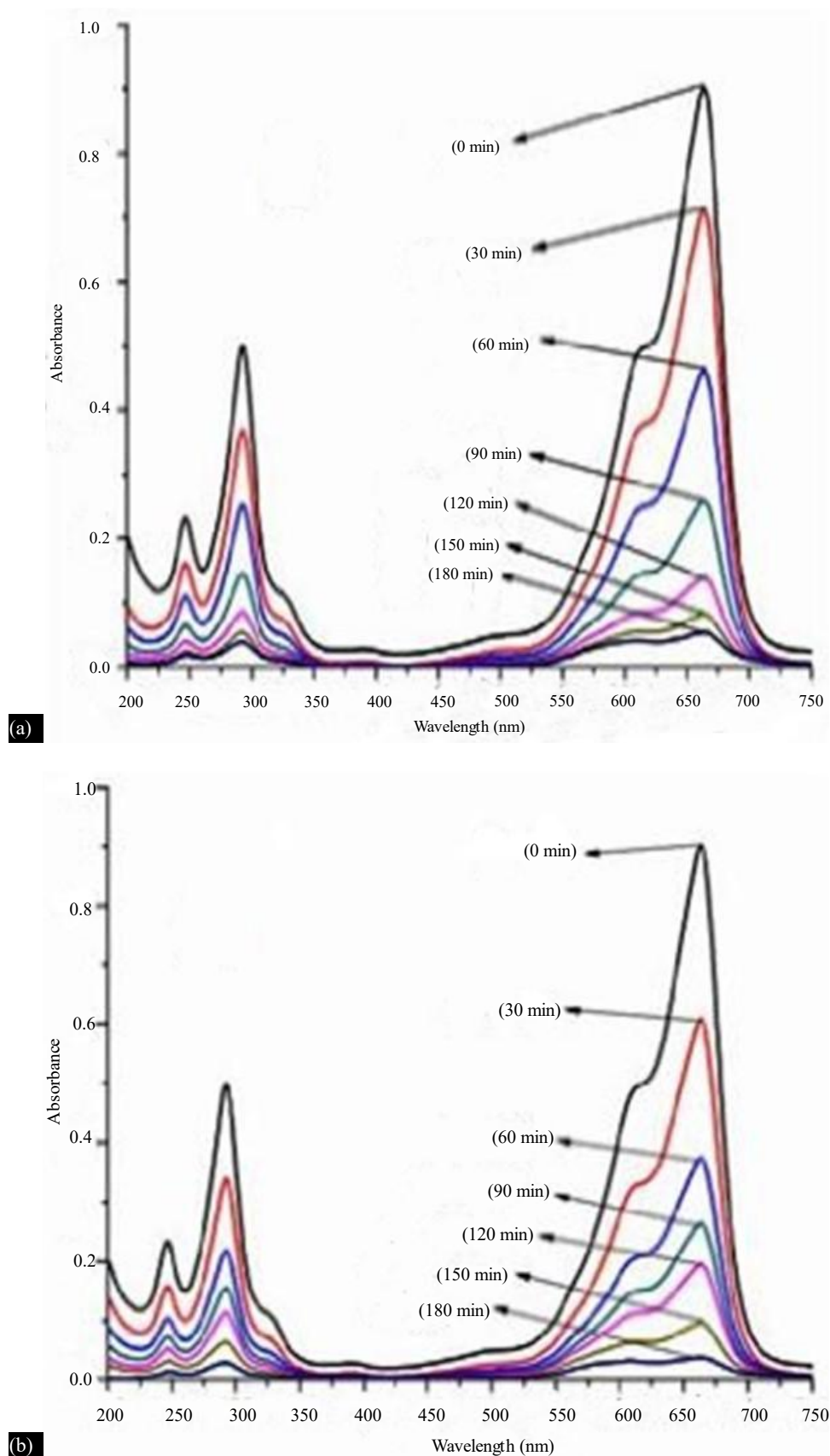
Figure 1. Absorbance spectral variations of blue -Methylene & Brhodamine by means of Cobalt Sulfide in Figure 1.a & 1.b and cobaltiron sulfide.
