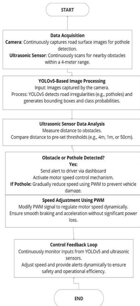
Figure 2: Flow chart describing the flow of working of the project
