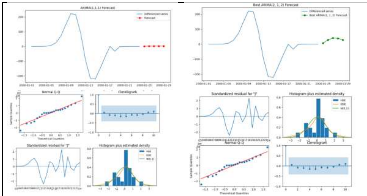
Figure 2: ARIMA model Forecast Comparison
