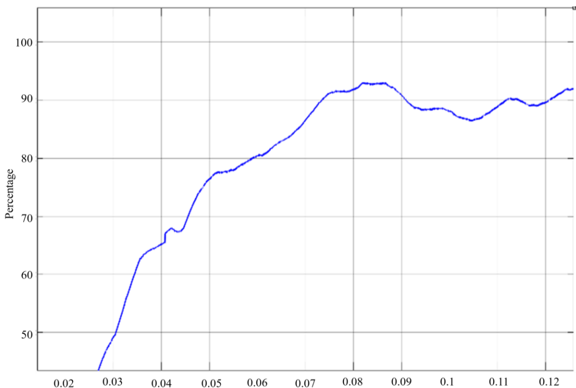
Figure 11. Efficiency curve.
