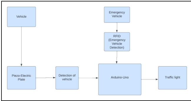
Figure 5. Block Diagram as per proposed system.
