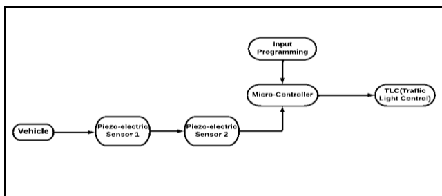
Figure 3. Density Measurement using Piezoelectric Material
