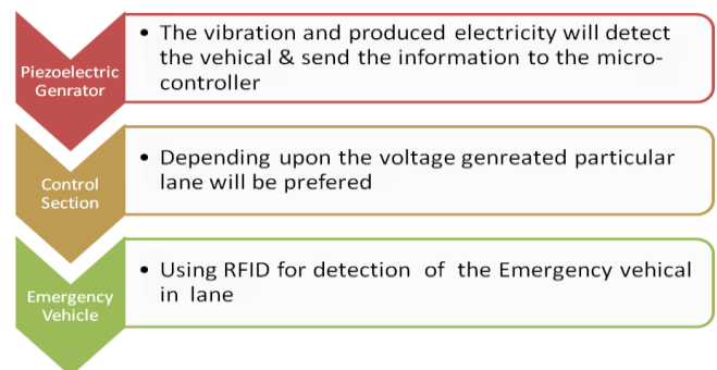
Figure 3. Density Measurement using Piezoelectric Material
