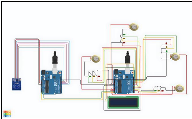
Figure 6. Circuit Diagram in the form of 2D model.
