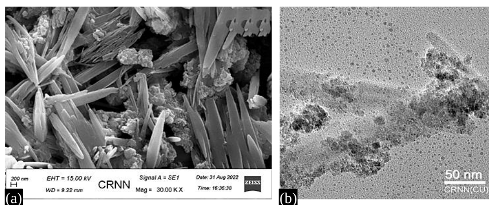
Figure 4. (A) SEM and (B) TEM Image of \text{Fe}_3\text{O}_4@\text{ISNA}@\text{NiL} .
