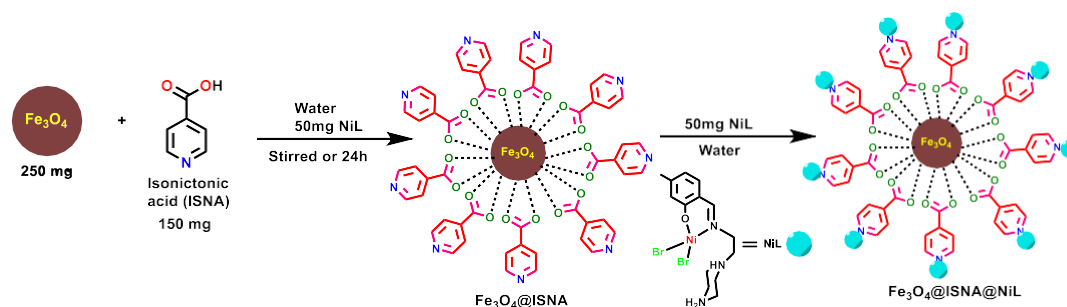
Figure 1. Schematic Representation for the Preparation of \text{Fe}_3\text{O}_4\text{@ISNA@NiL} .
