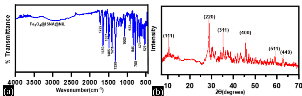
Figure 3. (A) FT-IR Spectrum Data and (B) PXRD Data of \text{Fe}_3\text{O}_4@\text{ISNA}@\text{NiL} .
