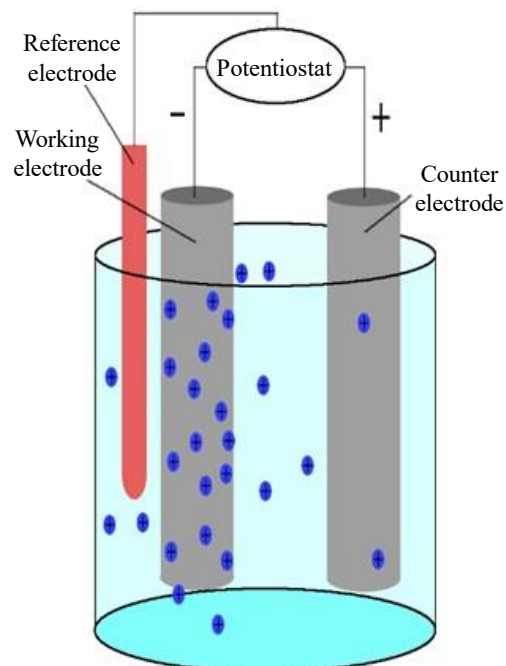
Figure 6. Electrochemical deposition coating process [17].
