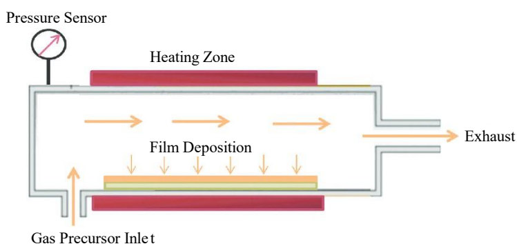
Figure 8. Chemical vapour deposition coating process [17].
