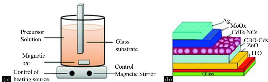
Figure 12. Wet-chemical coating process [25].
