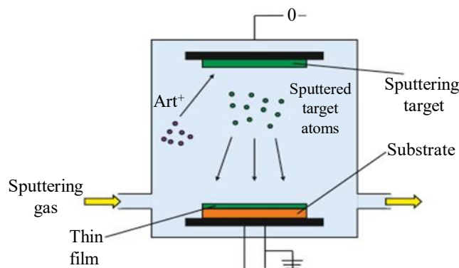
Figure 3. Vapor Deposition coating process [14].
