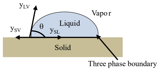
Figure 17. Forces operating at a liquid's three-phase contact line with a solid surface [60].
