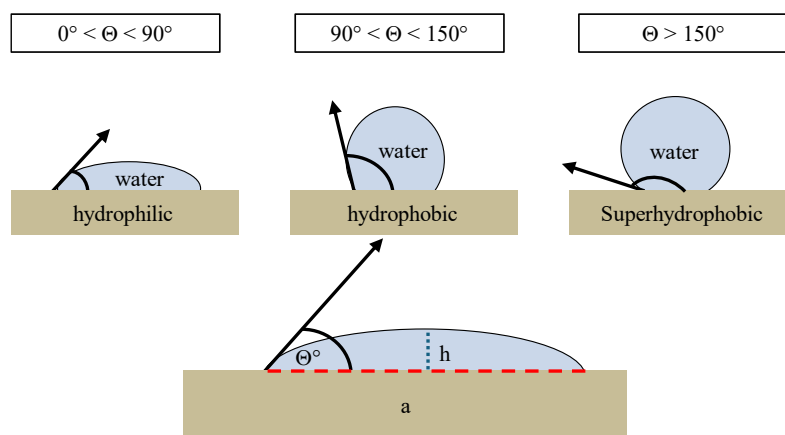
Figure 16. Contact angle range from hydrophilic to super hydrophobic [12].
