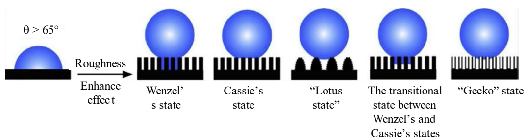
Figure 19. Water droplets in various stages on a solid surface [62].
