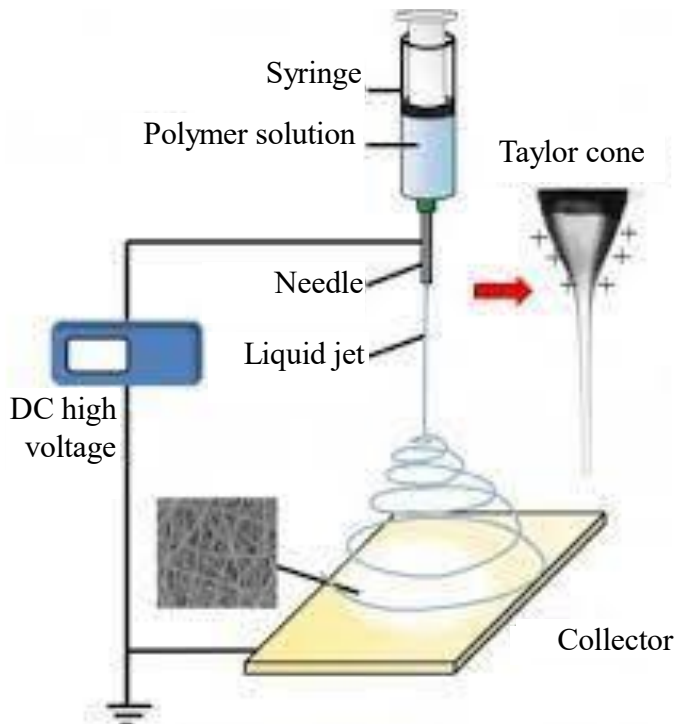
Figure 9. Electro spinning coating process [19].
