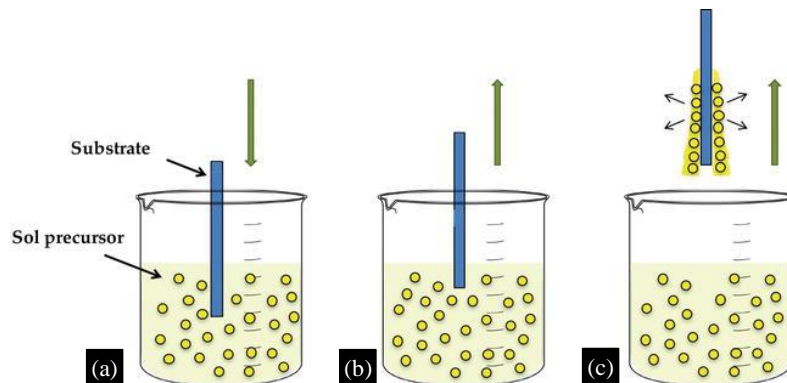
Figure 5. Sol-Gel coating process [16]. (a) Dipping (b) Deposition and Drainage (c) Evaporation.
