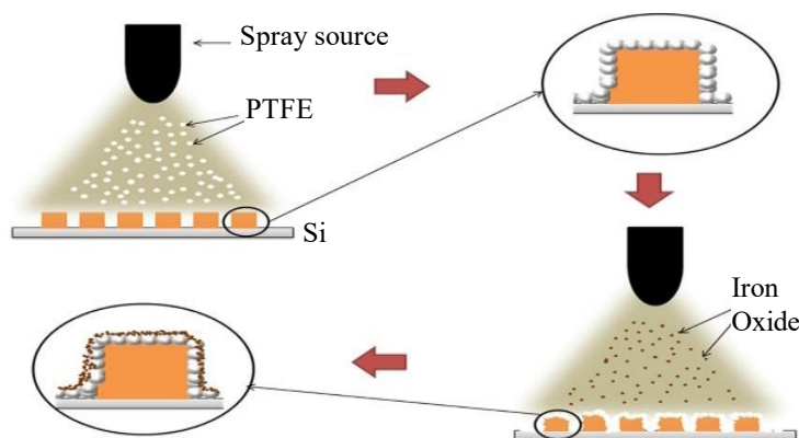
Figure 13. Lithography technique coating process [26].
