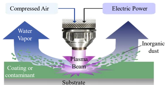
Figure 11. Plasma Treatment coating process [24].
