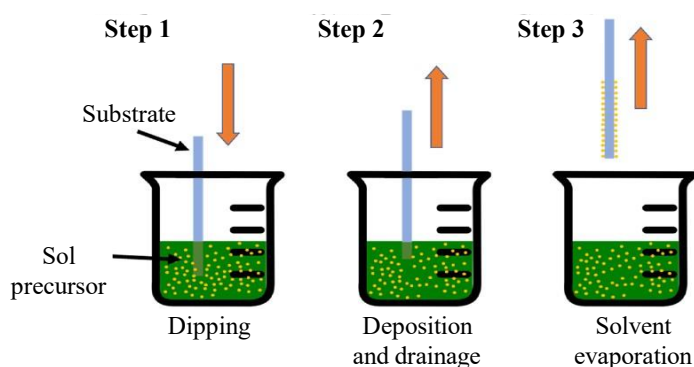
Figure 7. Solution immersion coating process [15-16].
