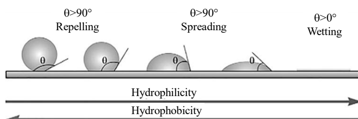
Figure 1. Diagram showing water droplet shape and water contact angle (WCA) for solid surfaces along hydrophobic and hydrophilic gradients [3].
