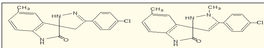
Fig.3 : Hydrazine Derivatives as Antibacterial Compounds.
