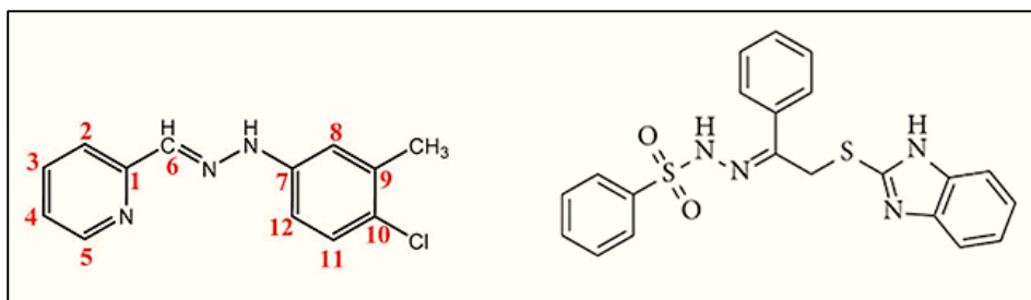
Fig.4 : Hydrazine Derivatives as Antimalaria Compounds.
