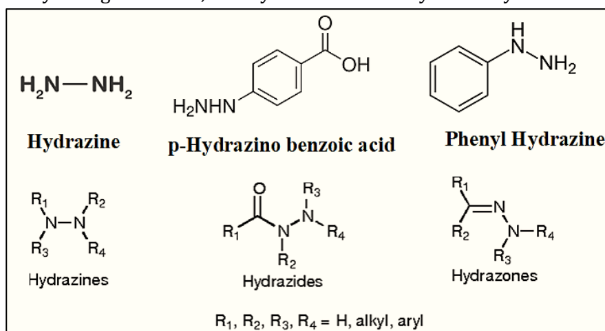
Fig. 1: Structures of Hydrazine Derivatives
