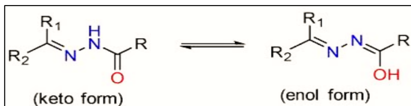
Fig. 2: Tautomerism Of Hydrazine Derivatives
