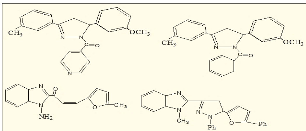
Fig.5 : Hydrazine Derivatives as Antitumor Compounds.
