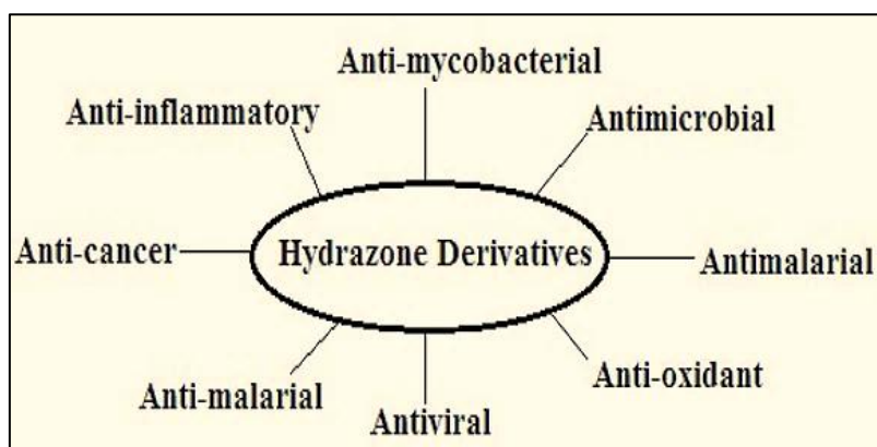
Fig. 7: Bio-Applications of Hydrazine
