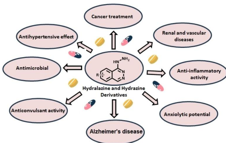
Fig. 8: Other Applications of Hydrazine
