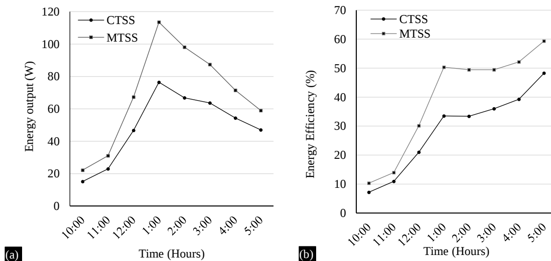
Figure 9. (a) and (b) Exergy Output and Exergy efficiency results CTSS and MTSS.
