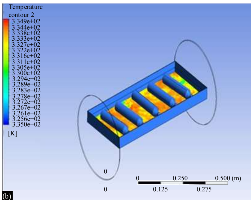
Figure 6. (a) and (b) Contours basin temperature at 2 pm CTSS and MTSS.
