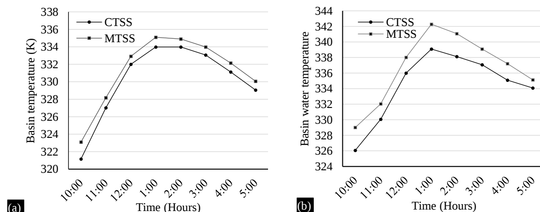
Figure 7. (a) and (b) Basin Temperature and basin water temperature CTSS and MTSS.
