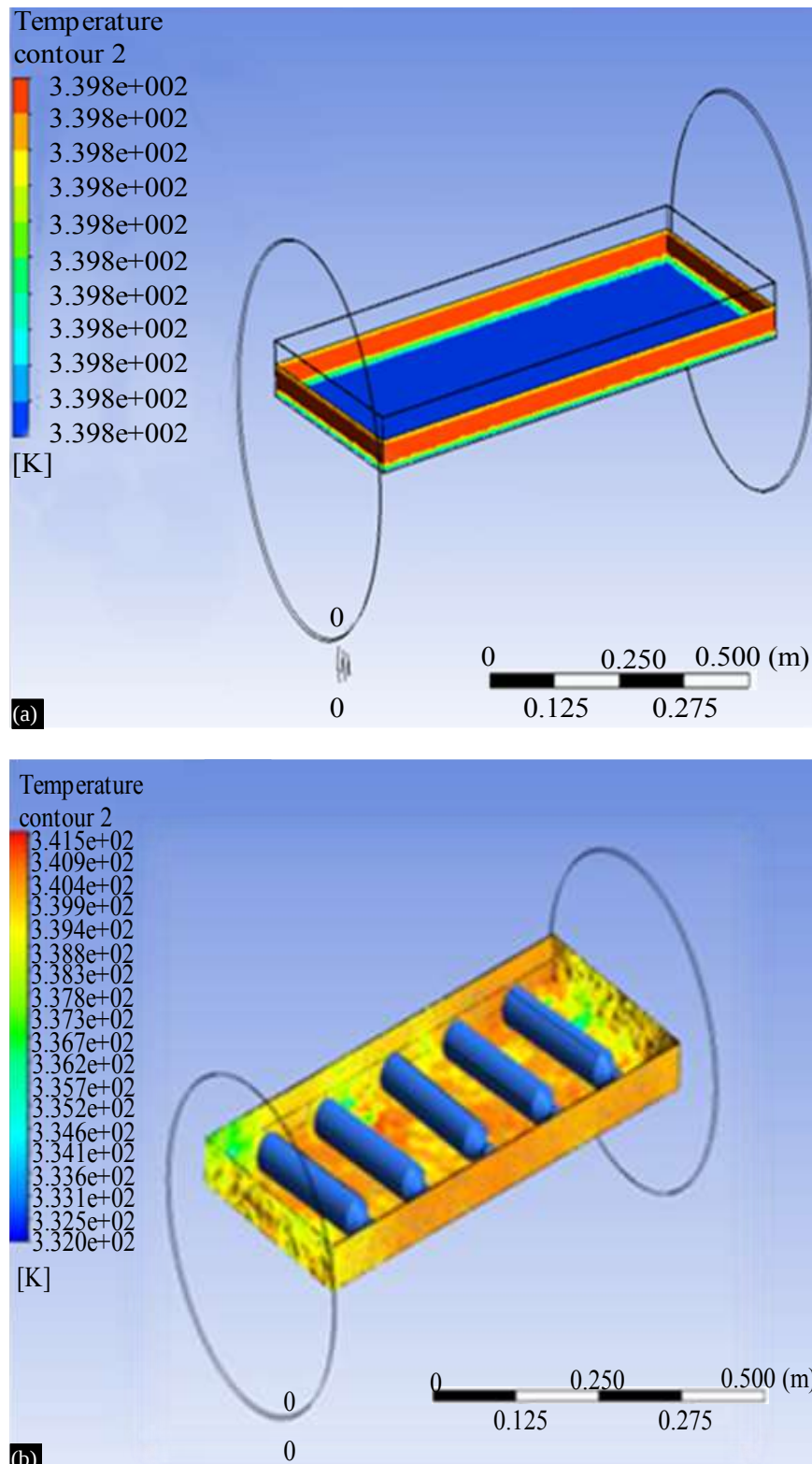
Figure 5. (a) and (b) Contours basin water temperature at 1 pm CTSS and MTSS.
