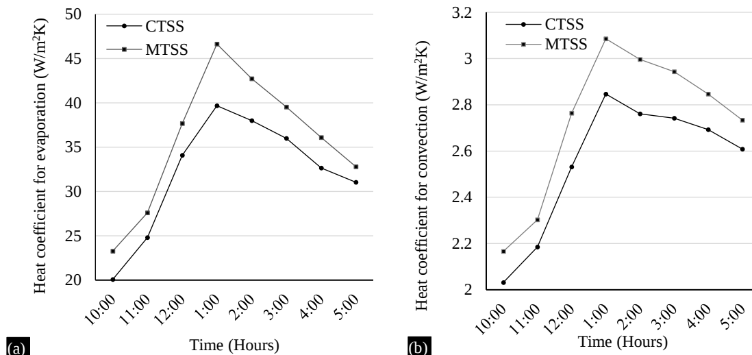
Figure 8. (a) and (b) Heat coefficient for evaporation and convection ( W/m^2K ) CTSS and MTSS.
