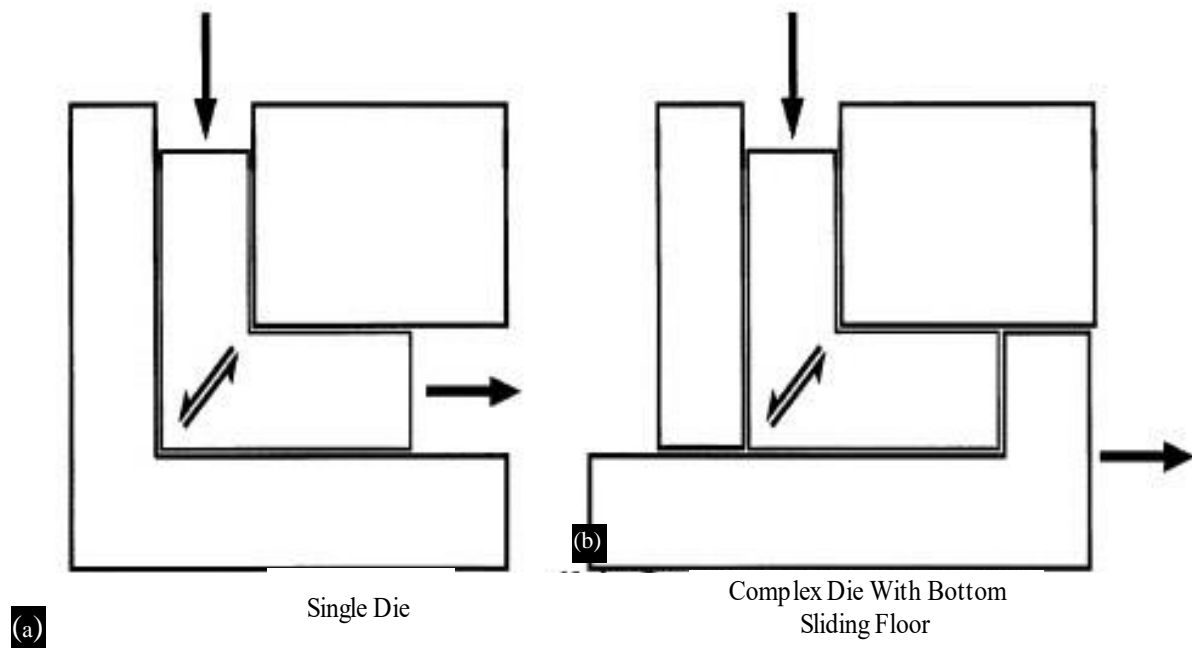
Figure 7. Geometry of ECAP Tooling with Simple Die and Complex Die with Bottom Sliding Floor [15].
