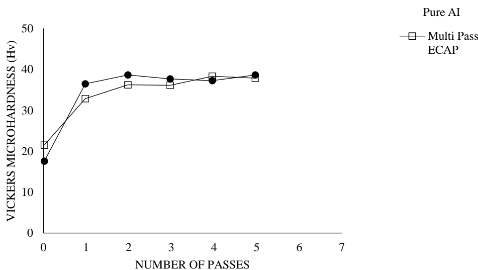
Figure 6. Number of Passes for Two Different Types of Samples [14].
