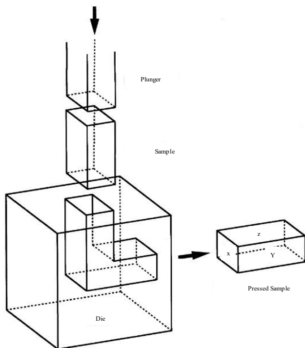
Figure 3. ECAP system, showing the x-planes, y-planes and z-planes with respected direction [8].
