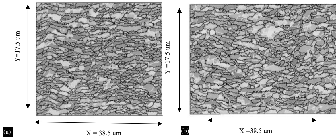
Figure 13. Displays High-Resolution EBSD Maps, which have been Cleaned, Capturing regions Near the End of the Billet [26].
