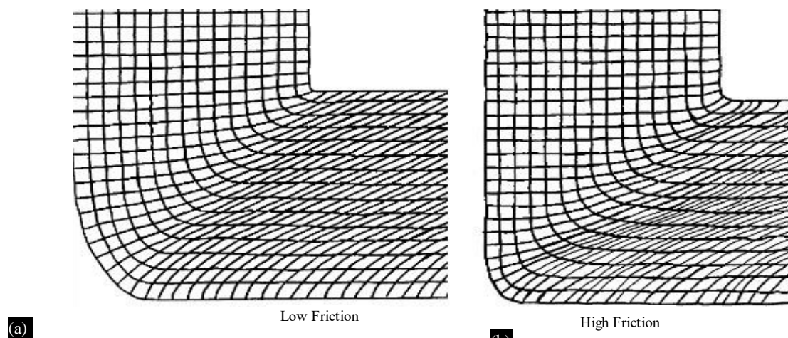
Figure 9. These Traces Correspond to Two Different Conditions at (a) Low Friction and (b) High Friction [19].
