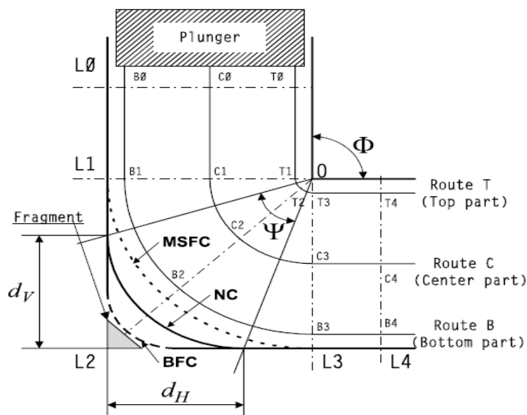
Figure 4. The Condition of the Corner During the ECAP Procedure [12].
