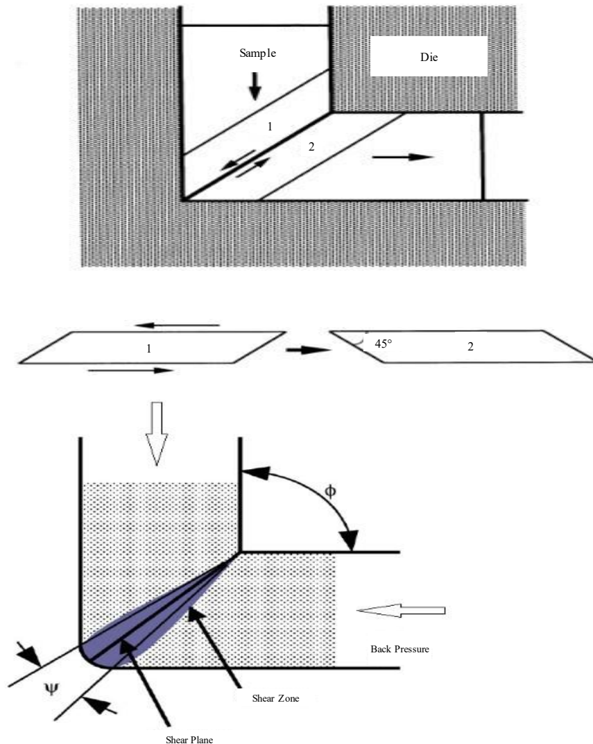
Figure 2. Shearing plane within the die of ECAP Process and Back Pressure [5].
