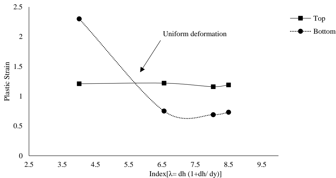
Figure 15. Corner Shape Index for Homogeneous Plastic Strain Distribution [30].
