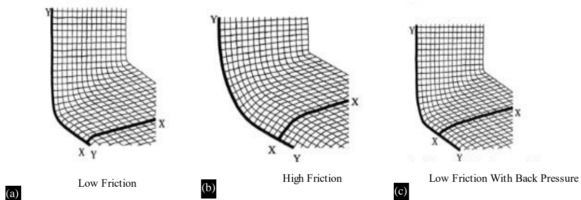
Figure 8. The Pressing Conditions Measured through (a) Low Friction, (b) High Friction, and (c) Low Friction with Back Pressure [18].
