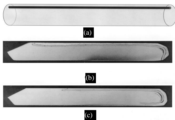
Figure 12. Displays Cross-Sectional Views of Billets Featuring Copper Wire Markers Through the 120^{\circ} die [25].
