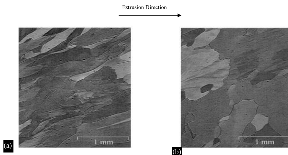
Figure 11. Underwent Deformation at Room Temperature Without Application of Back Pressure and Under Low Friction Conditions [24].
