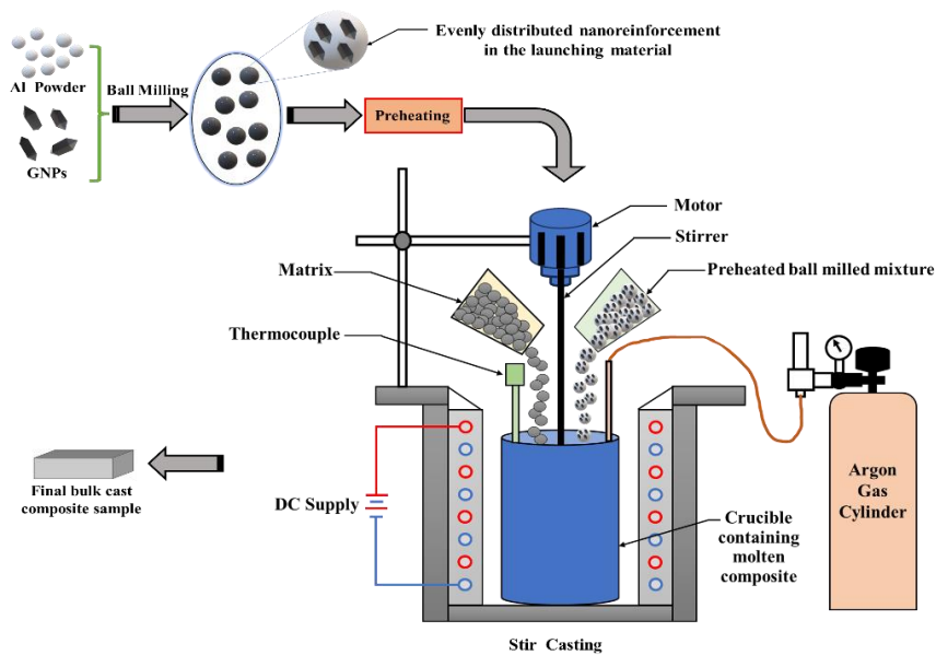
Figure 3. Combined liquid metallurgy (stir casting) and powder metallurgy (ball milling).
