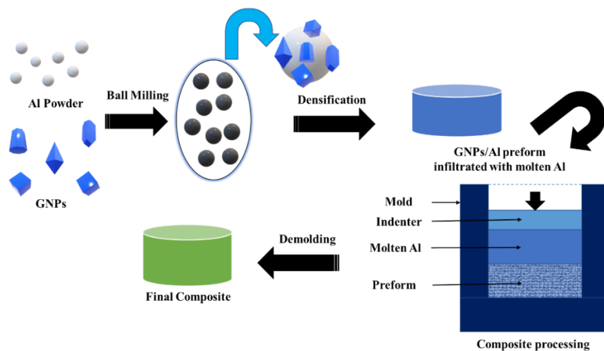
Figure 4. Combined ball milling and pressure infiltration.
