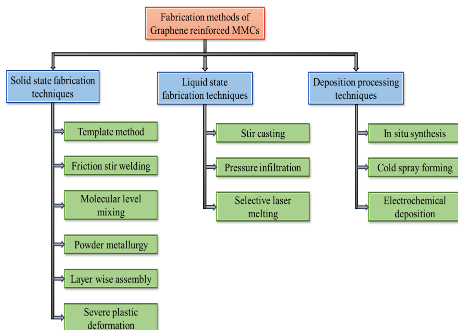
Figure 2. Several fabrication techniques for developing GNPs reinforced MMCs.
