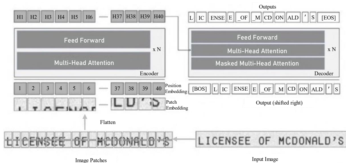
Figure 2. Implementing OCR with Transformer (TrOCR).
