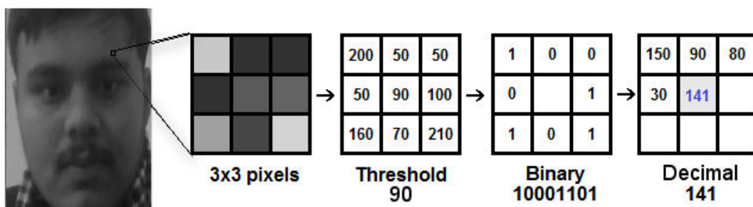
Figure 2. Performing local binary pattern (LBP) operation.
