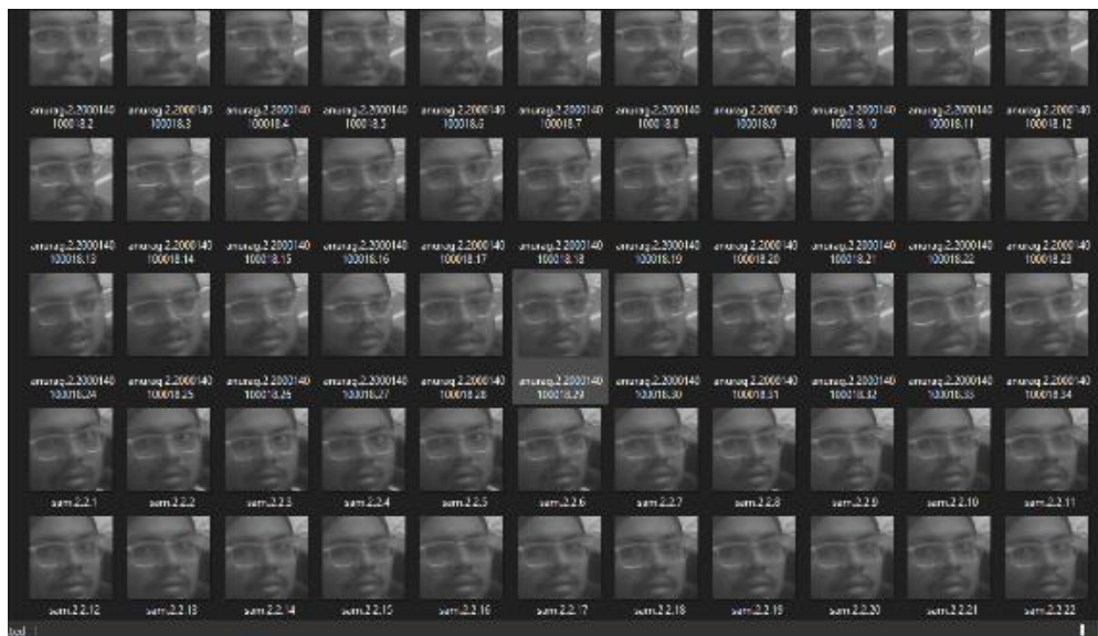
Figure 7. Trained dataset.
