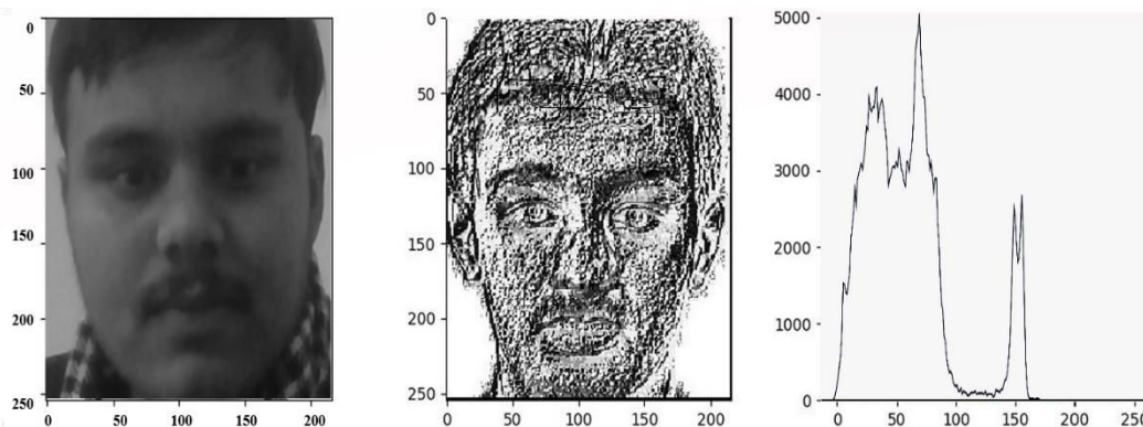
Figure 3. Extracting histogram.
