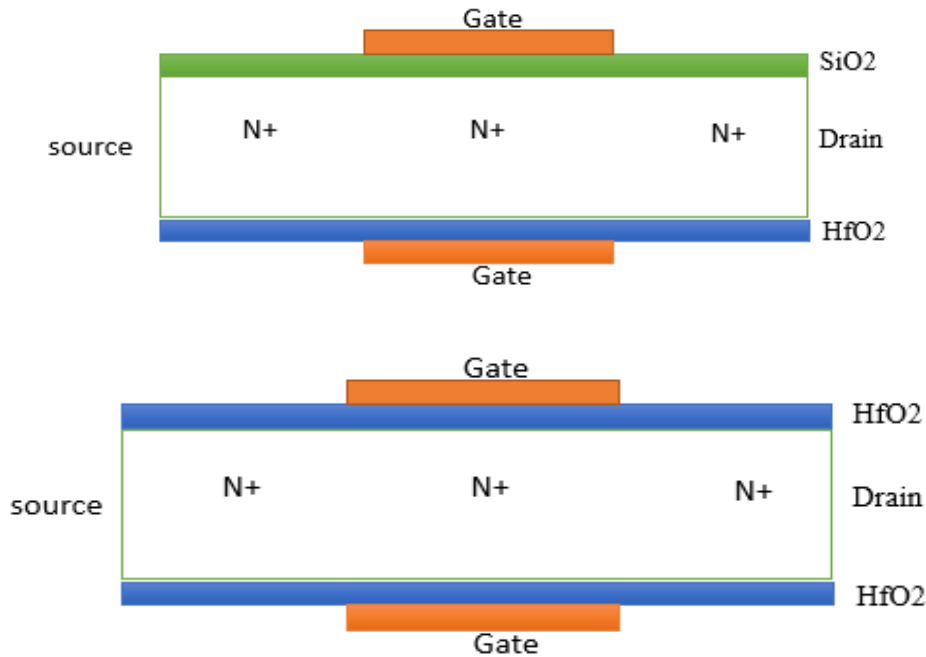
Figure 2. Schematic device structures of symmetric and asymmetric oxide JLFET with an EOT value of 1 nm and L_{\text{ch}} = 40 nm.
