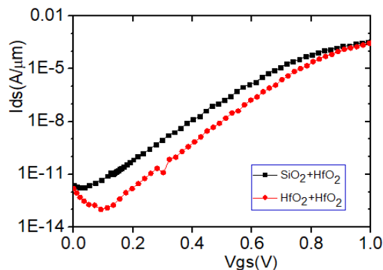
Figure 3. Measured output characteristics ( I_{\text{ds}}-V_{\text{gs}} ) of symmetric and asymmetric oxide JLFET ( V_{\text{ds}}=1\text{V} ).
