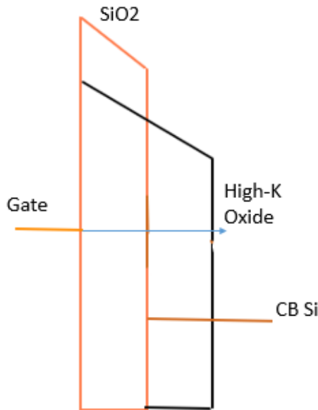
Figure 1. Graphic of Direct tunneling through SiO 2 and difficult tunneling through High-k Oxide (HfO 2 ).
