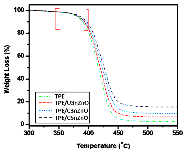
Figure 3. TGA curves of TPE and TPE/nZnO nanocomposites.
