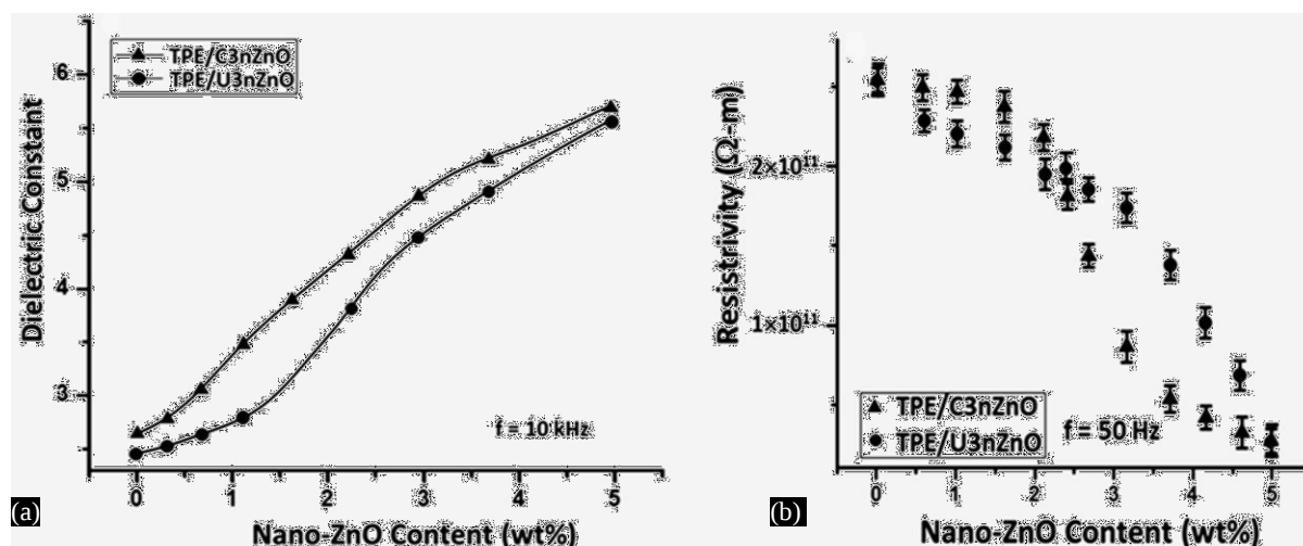
Figure 6. (a–b) (a) Dielectric constant and (b) Resistivity of TPE/nZnO nanocomposites as a function of nano-ZnO content (wt%).
