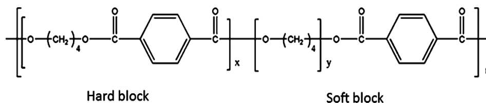
Scheme 1. Chemical structure of the thermoplastic polyester elastomer (TPE).
