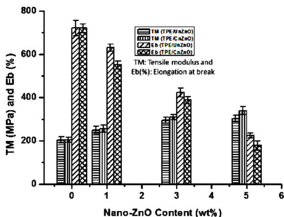
Figure 5. Tensile and elongation at break of TPE/nZnO nanocomposites.
