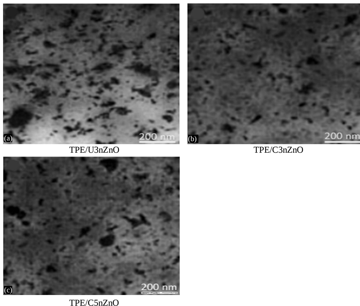
Figure 1. (a–c) TEM photomicrographs of TPE/nZnO nanocomposites (w/w%) (a) TPE/U3nZnO, (b) TPE/C3nZnO, (c) TPE/C5nZnO.
